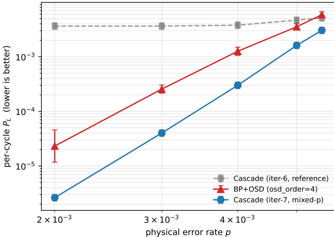
BB-[[144,12,12]] iter-7 (mixed-p): Cascade vs BP+OSD
