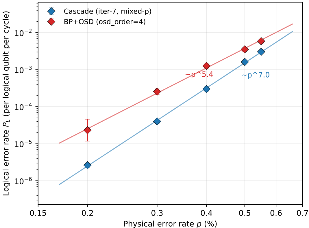
BB-[[144,12,12]]: Cascade (iter-7, mixed-p) vs BP+OSD
