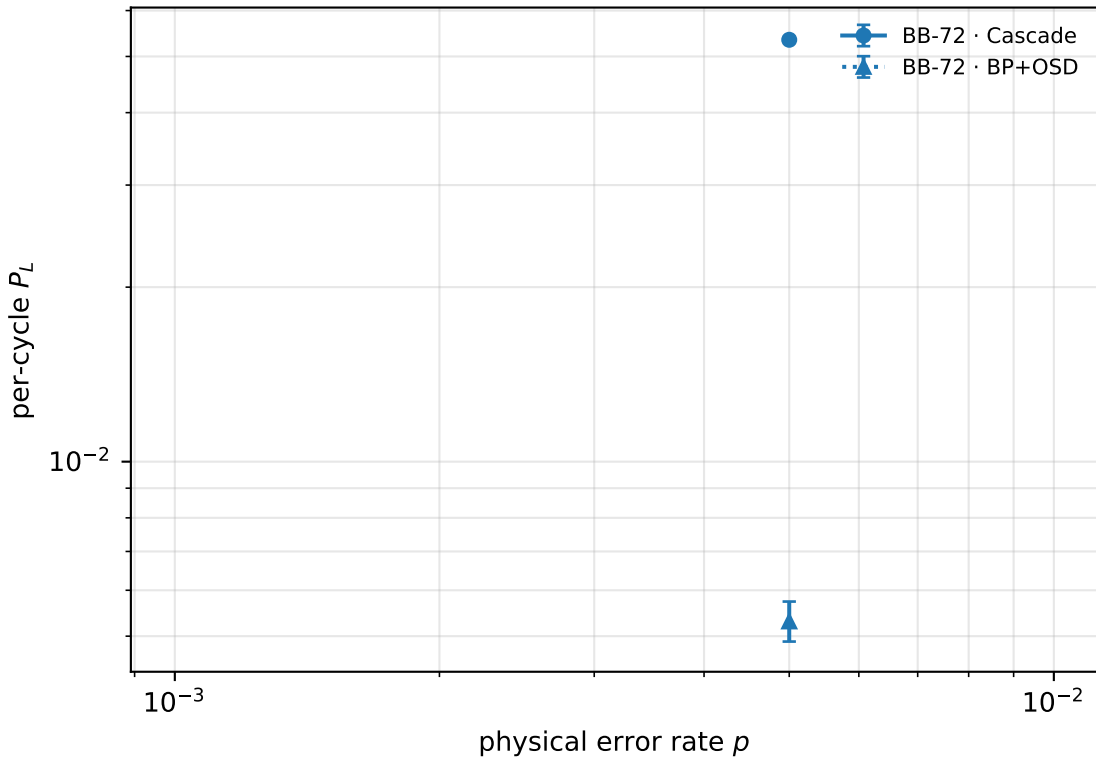
BB-72: Cascade (iter-2) vs BP+OSD
