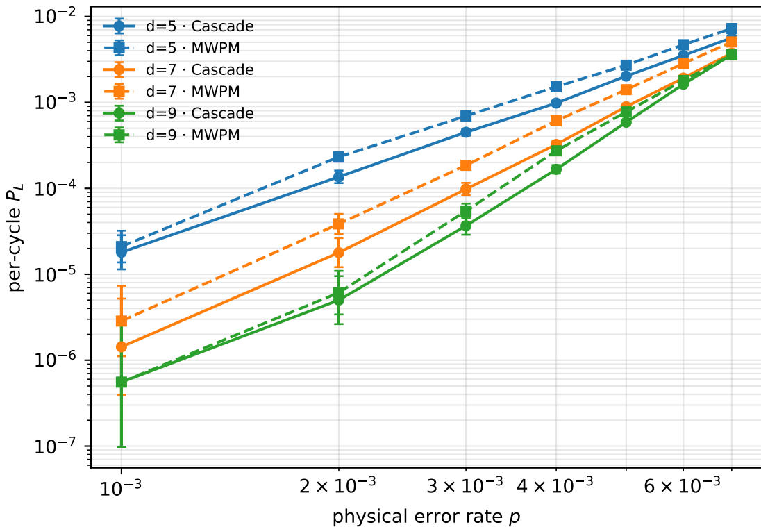
Surface code: Cascade (H=128) vs MWPM
