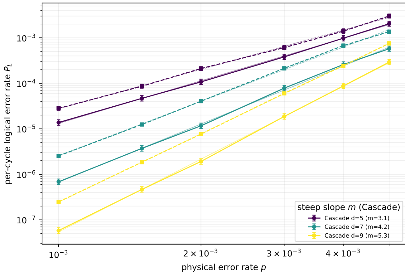
Surface-code waterfall: Cascade (solid) vs MWPM (dashed)
