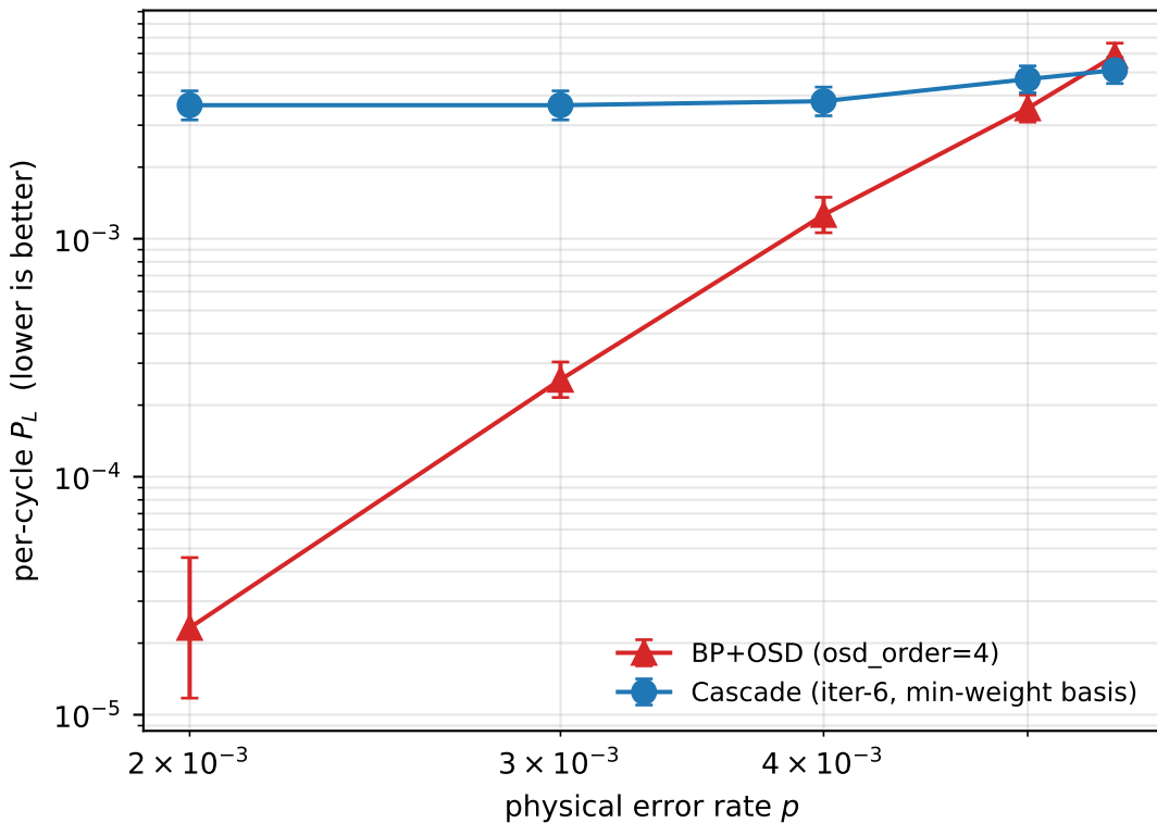
BB-[[144,12,12]] iter-6: Cascade vs BP+OSD
