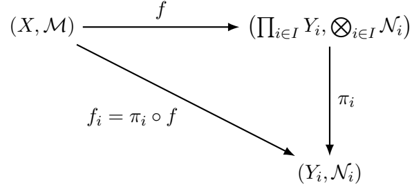
FIGURE 3. Measurability into a product can be checked one coordinate at a time.
