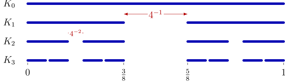
FIGURE 2. The first stages of the fat Cantor construction. The deleted intervals become shorter quickly enough that the limiting set retains measure 1/2 .
