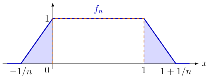
FIGURE 12. The two shaded triangles give the L^1 distance from f_n to \mathbf{1}_{[0,1]} . Their total area is 1/n .
