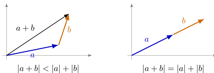
FIGURE 10. Different complex phases cause cancellation. Equality in the integral triangle inequality requires a common phase almost everywhere, as in the aligned vectors on the right.
