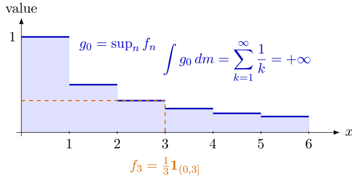
FIGURE 11. The envelope of f_n = n^{-1}\mathbf{1}_{(0,n]} has a divergent harmonic tail. Every f_n is integrable, but no single integrable function dominates the sequence.
