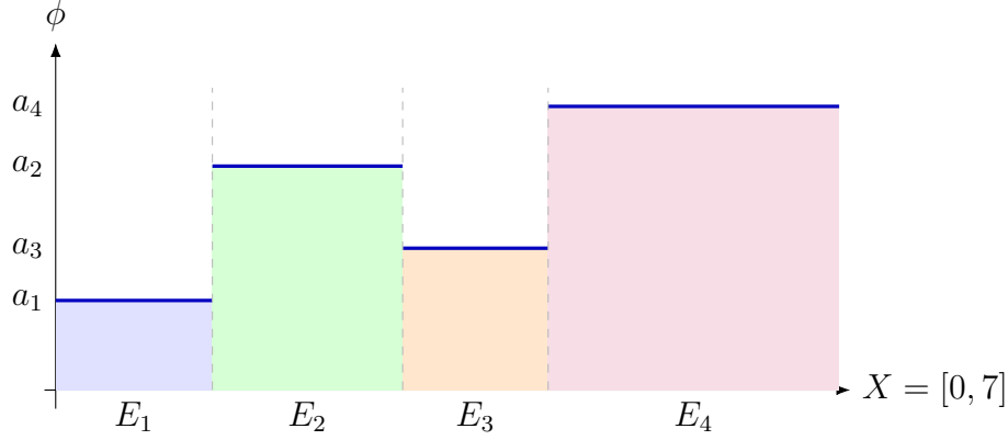
FIGURE 5. A simple function \phi = \sum_{j=1}^4 a_j \mathbf{1}_{E_j} in standard form. The sets E_j need not be intervals in a general measurable space.
