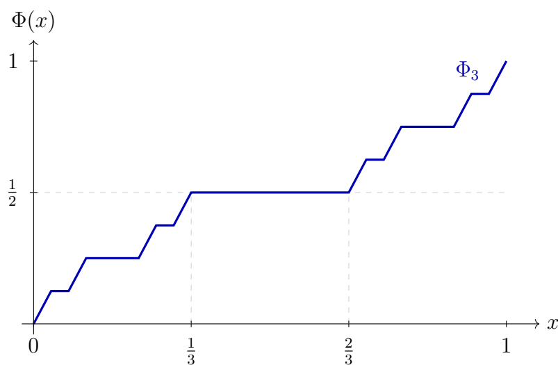
FIGURE 1. The third-stage polygonal approximation \Phi_3 to the Cantor function. At every subsequent stage, each sloping segment is replaced by a smaller copy of the first-stage pattern; the limit is constant on every component of [0, 1] \setminus C .
