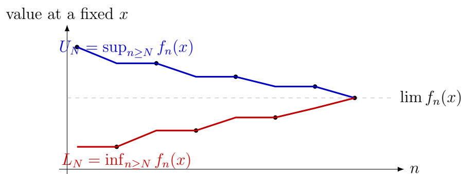
FIGURE 4. The tail supremum decreases and the tail infimum increases. Their limits are the pointwise lim sup and lim inf; the drawing shows the convergent case.
