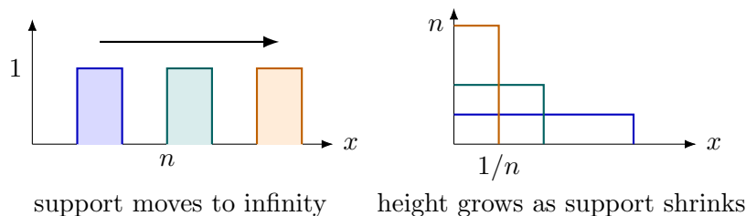
FIGURE 9. Each rectangle has area 1, but both pointwise limits are zero. Endpoint values do not affect these Lebesgue integrals.
