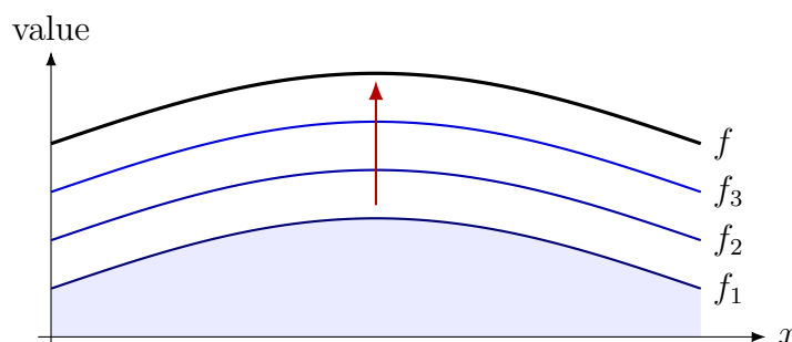
FIGURE 8. For an increasing sequence of nonnegative functions, the regions below the graphs increase to the region below the limit. The monotone convergence theorem makes this area intuition valid on an arbitrary measure space.
