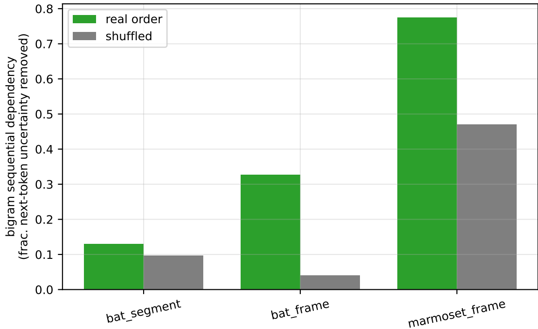
Sequential dependency: marmosets \gg bats (mechanism)
