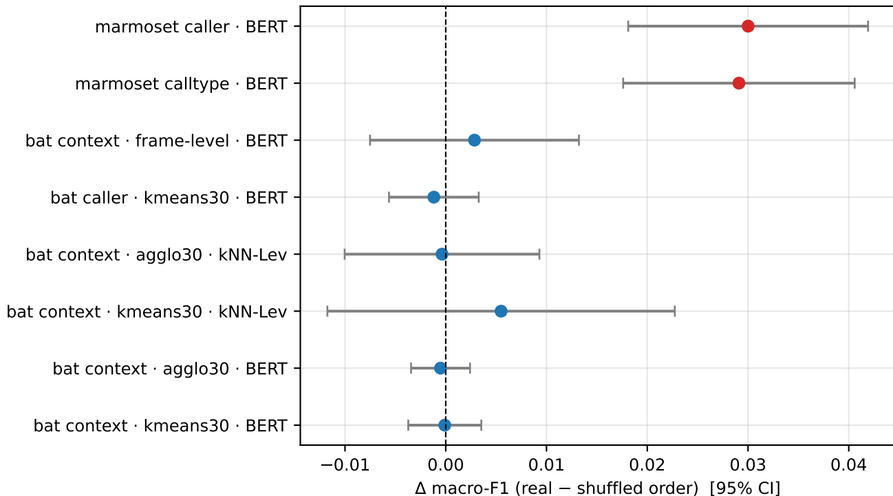
Token order ablation: bats (blue) vs marmosets (red)
