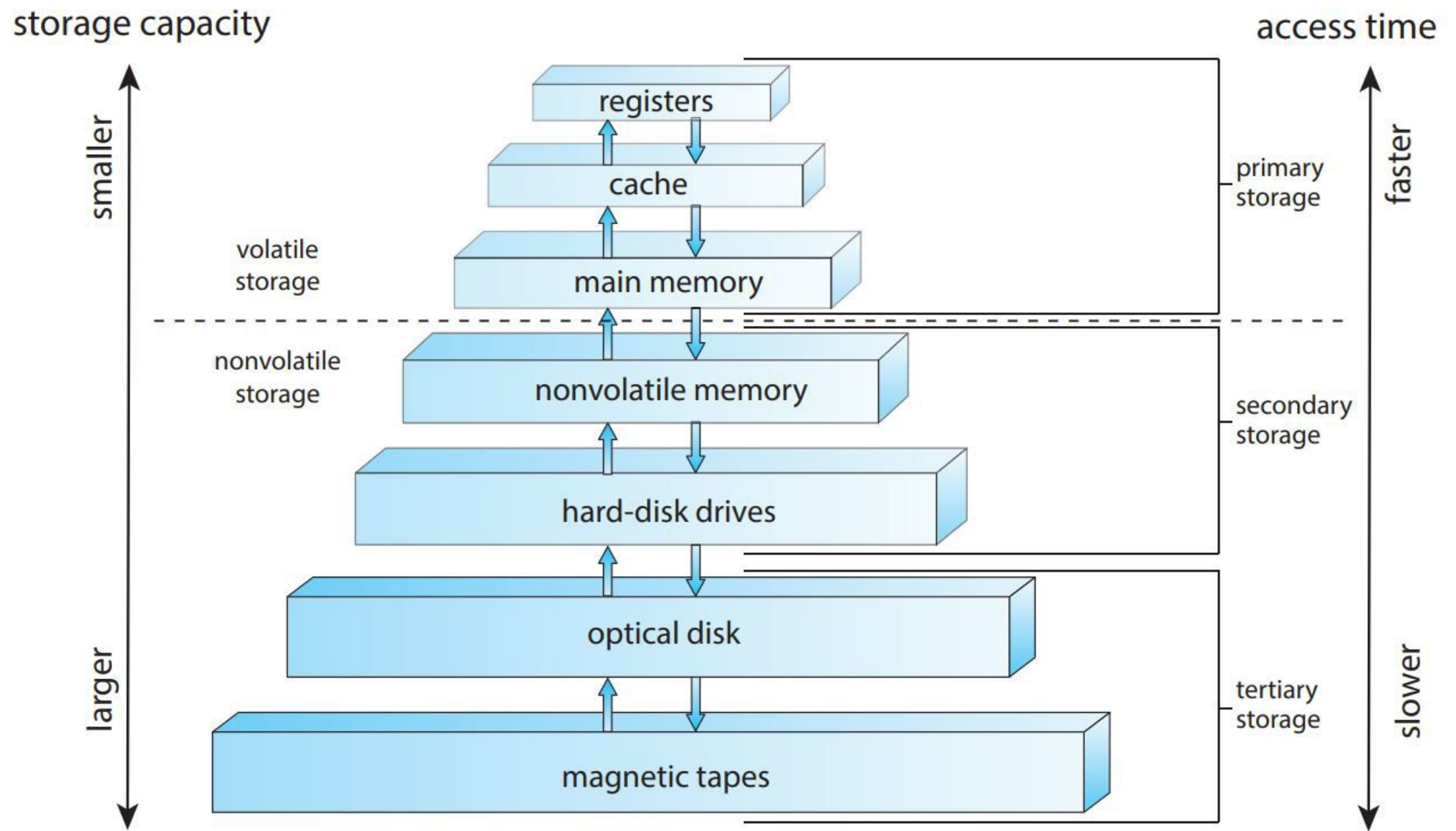
Figure 1.6 Storage-device hierarchy.
