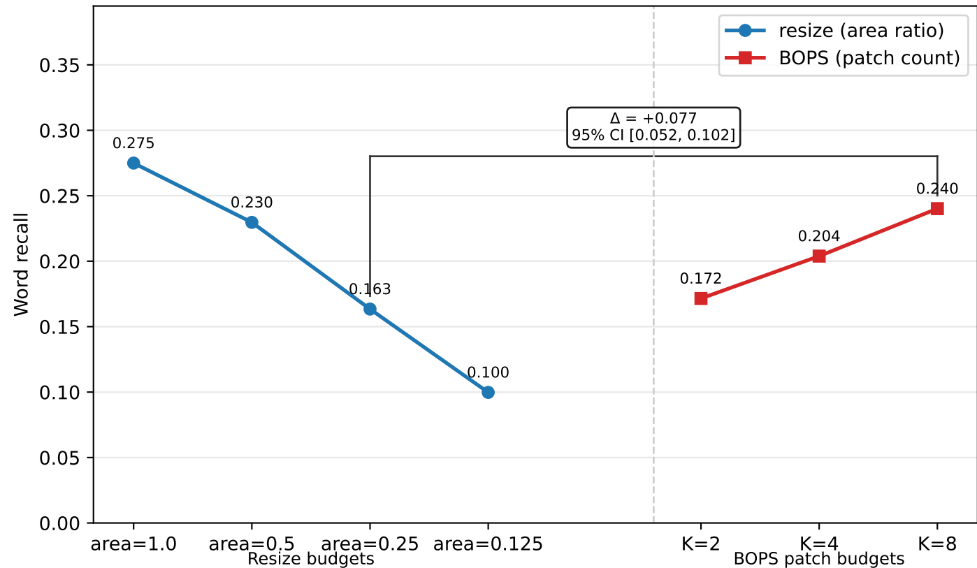
OCR word recall vs visual budget (TextOCR pilot, n=200)
