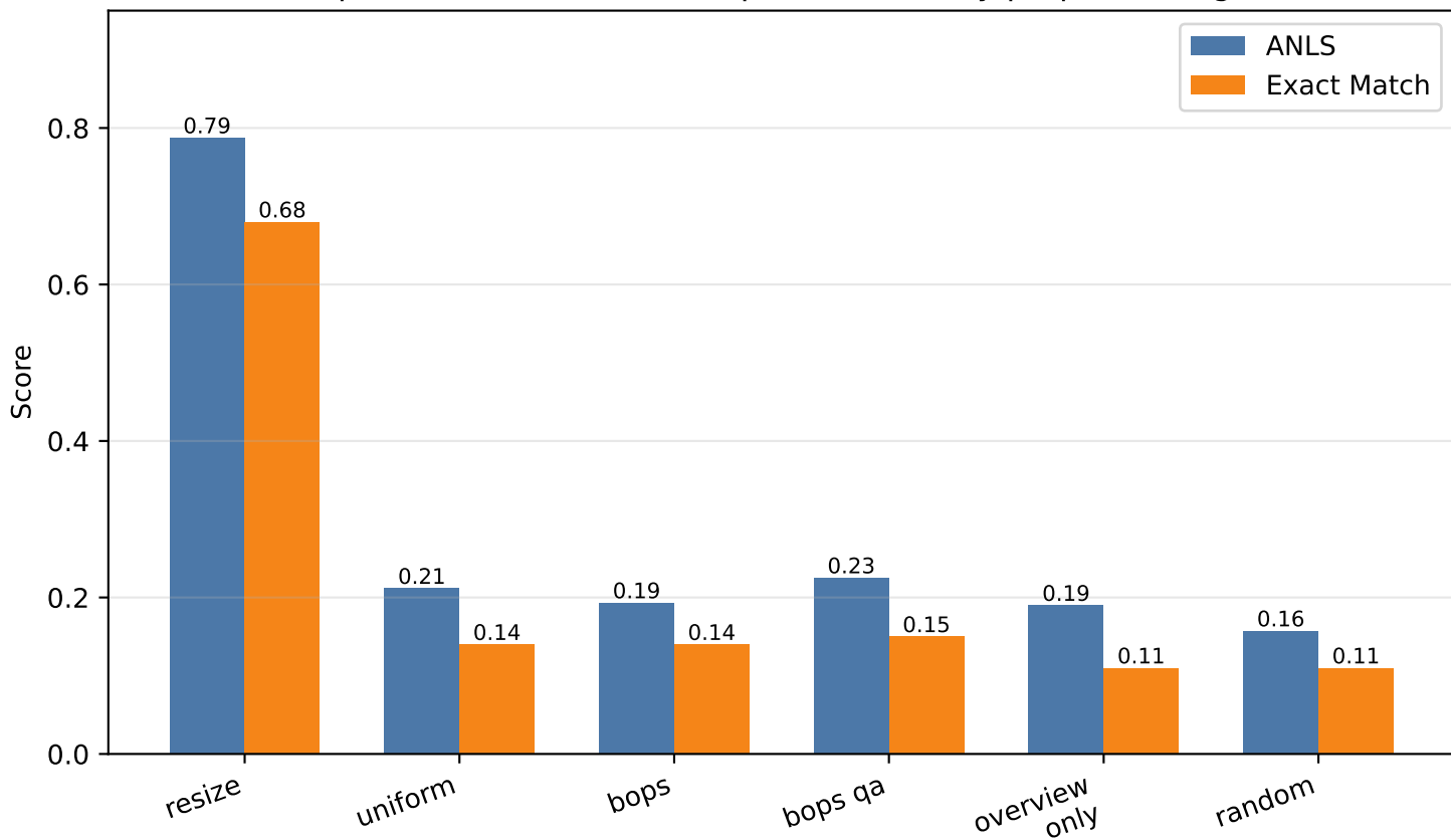
DocVQA pilot (n=100, K=2): VLM performance by preprocessing method
