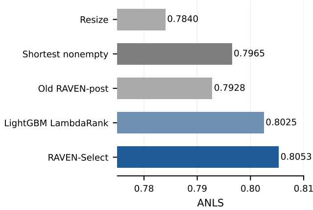
Fig. 2. Primary ANLS comparison on DocVQA n = 500 . RAVEN-Select’s paired improvement is +0.0214 over resize (95% CI [+0.0062, +0.0380]) and +0.0088 over shortest nonempty (95% CI [+0.0023, +0.0173]).
