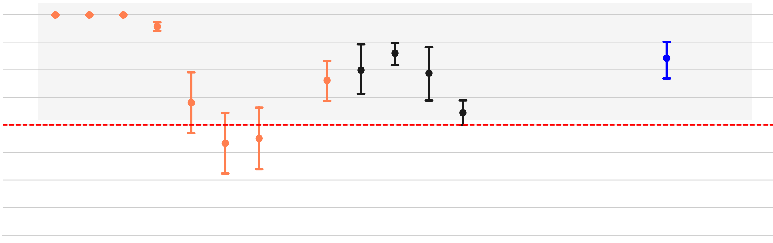
Mistral-Small-3.2
