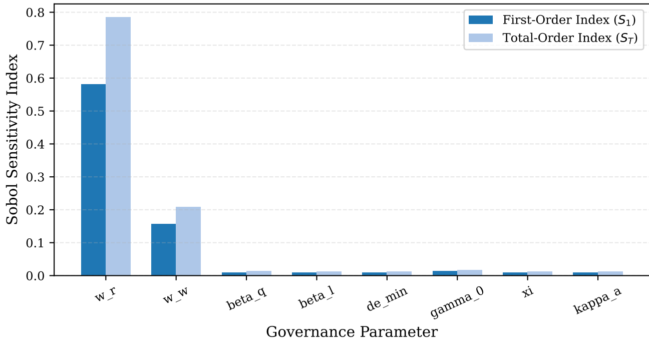
Global Sobol Sensitivity Variance Decomposition
