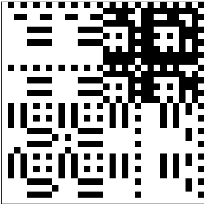
5-strategy S_{5,5} winning prob. 358/1024
