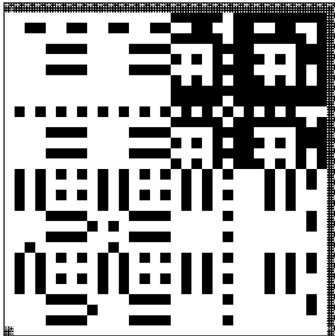
Strategy S_5 winning prob. = 7/20
