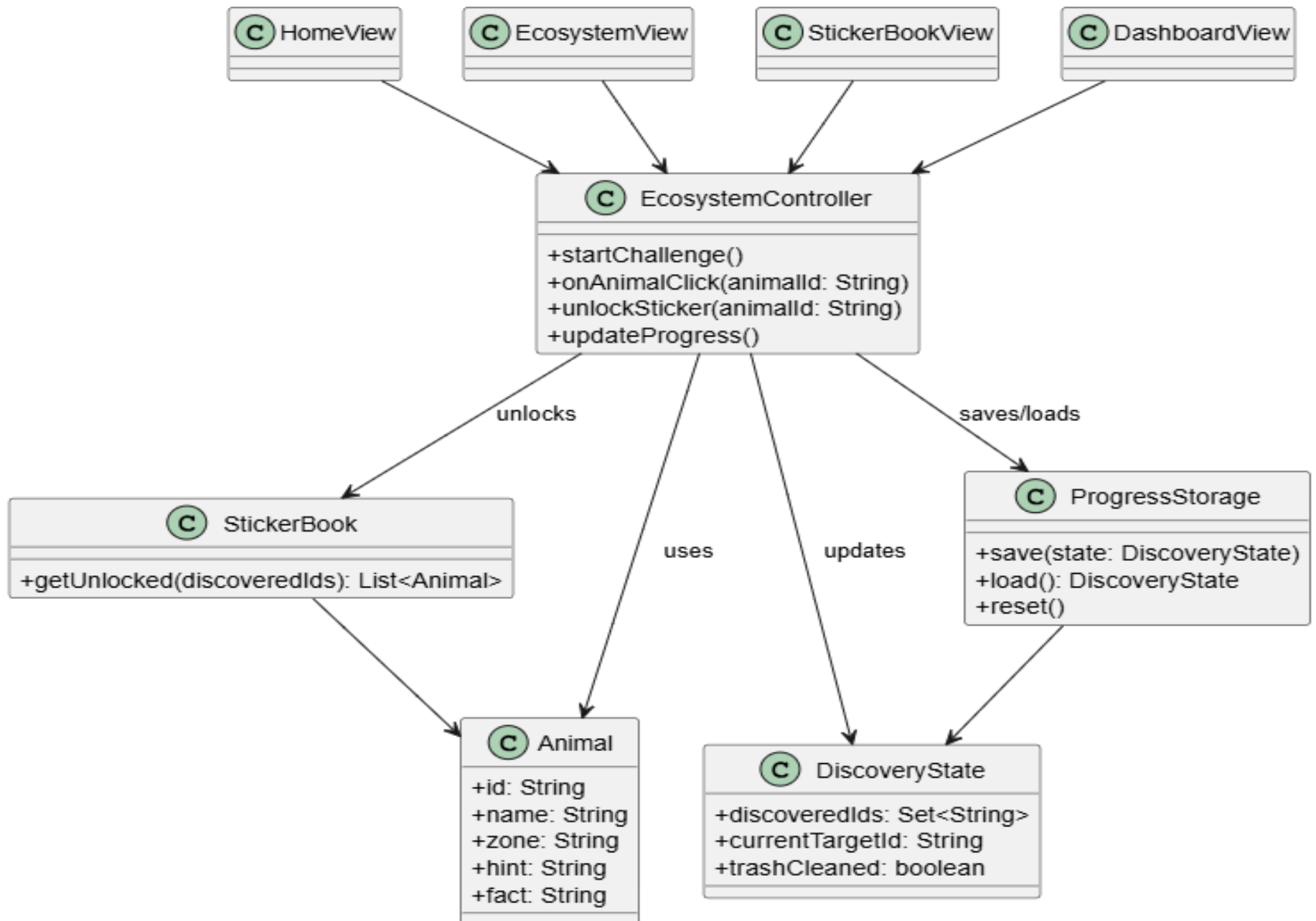
EcoDiscovery - Simple Class Diagram (Core System)
