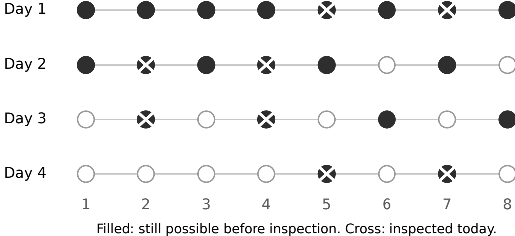
Figure 6: An optimal four-day search of eight rooms with two daily probes. The rows show every position still possible before that day's inspection.
