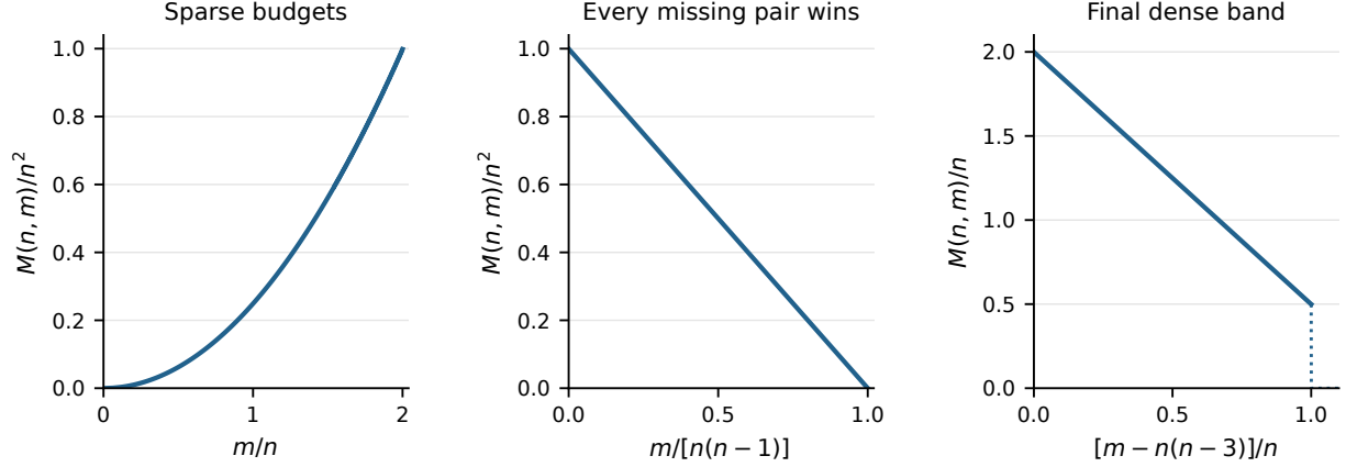
Figure 1: The three exact regimes at n = 1800 : sparse growth, the main interval, and the final dense band. Separate axis scales show the two narrow endpoint regimes. The dotted continuation in the last panel leads to zero above n(n-2) .
