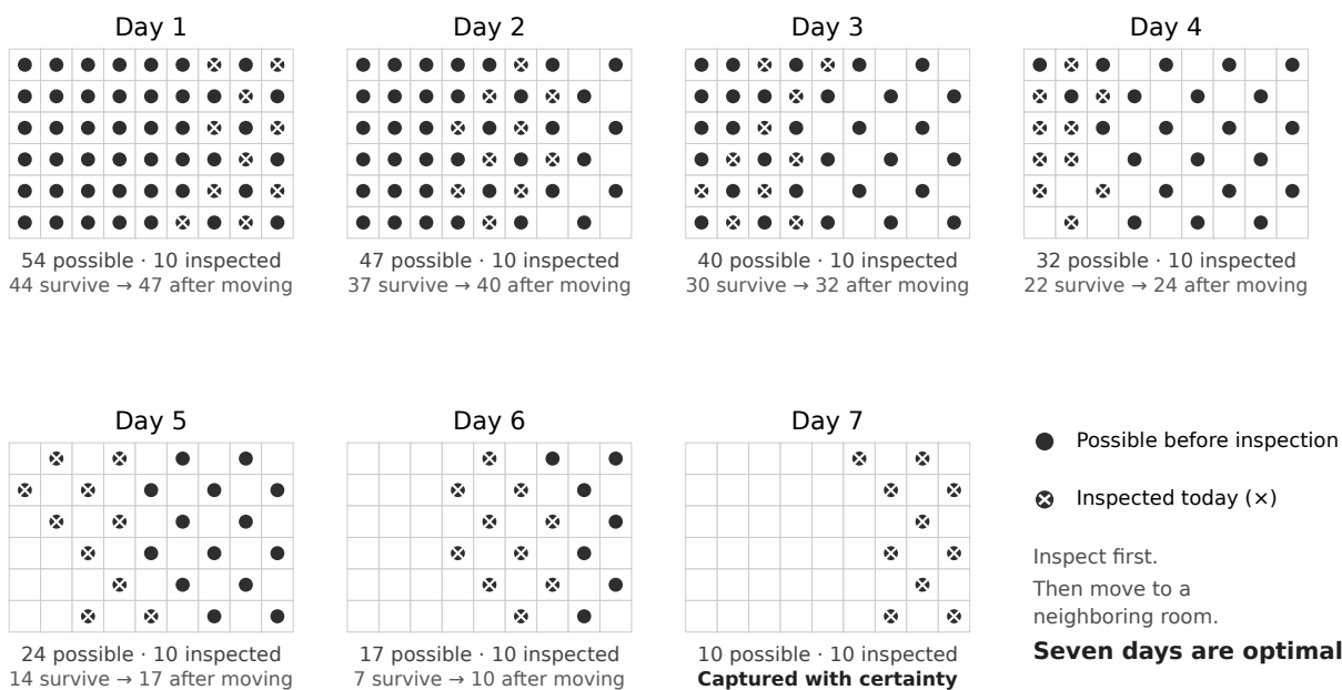
Figure 3: An optimal seven-day search on 6 \times 9 with ten daily inspections, constructed backwards from the final survivor envelope. Every displayed possible-position set and inspection has been replayed on the physical room graph.
