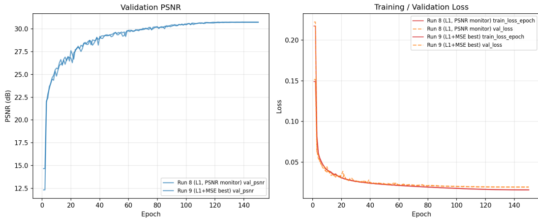
Figure 2: Training and validation curves for Run 8 (L1 loss, PSNR-monitored) and Run 9 (L1+MSE, \lambda = 0.05 ). Left: validation PSNR plateaus around epoch 80–100 for both runs, with Run 9 achieving a slightly higher best val_psnr (30.749 vs 30.718). Right: training and validation loss curves converge without overfitting; Run 9’s training loss tracks slightly below Run 8’s.
