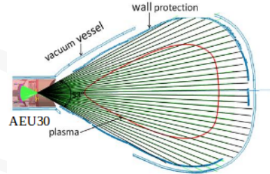
horizontal bolometer camera (HBC)
