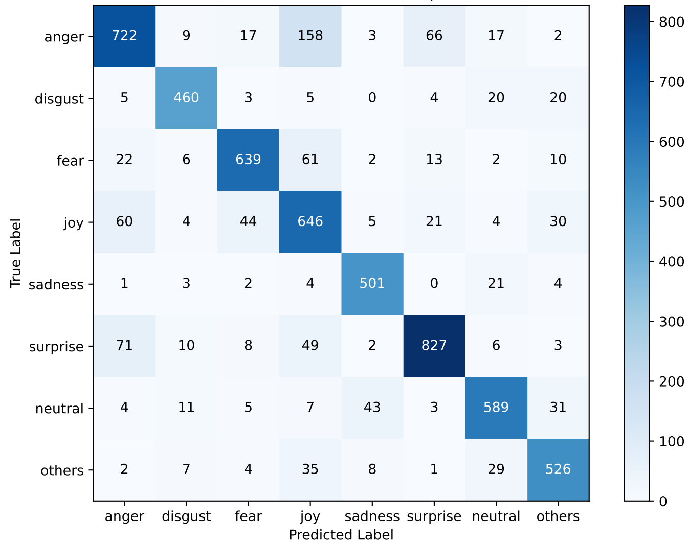
Emoset - Confusion Matrix (Epoch 2)
