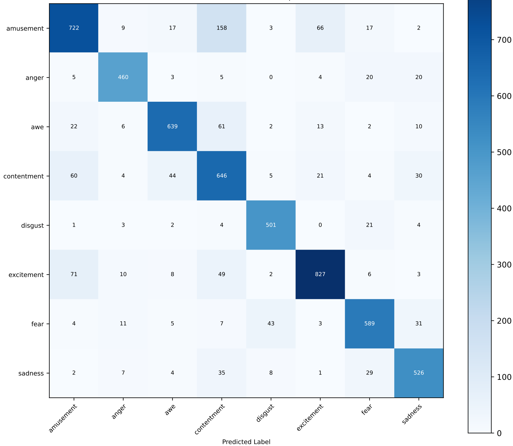
Emoset - Confusion Matrix (Epoch 2)
