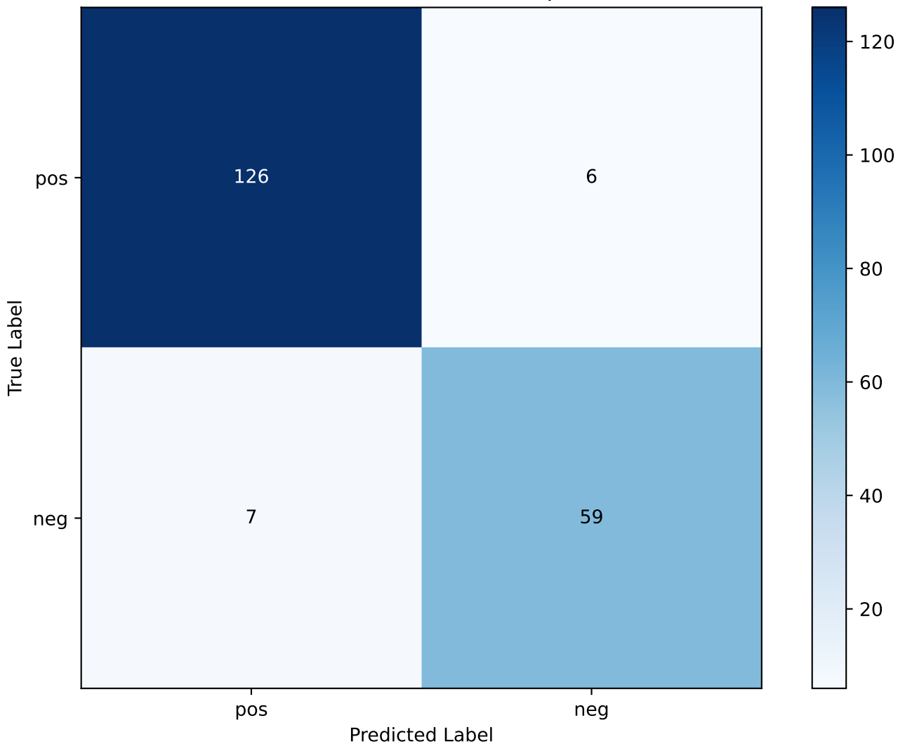
Emotion6 - Confusion Matrix (Epoch 24)
