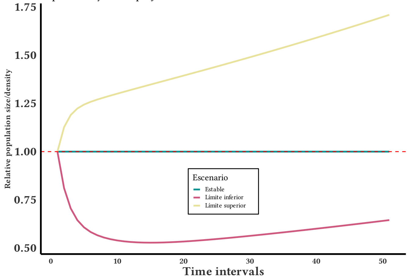
Population dynamics projections
