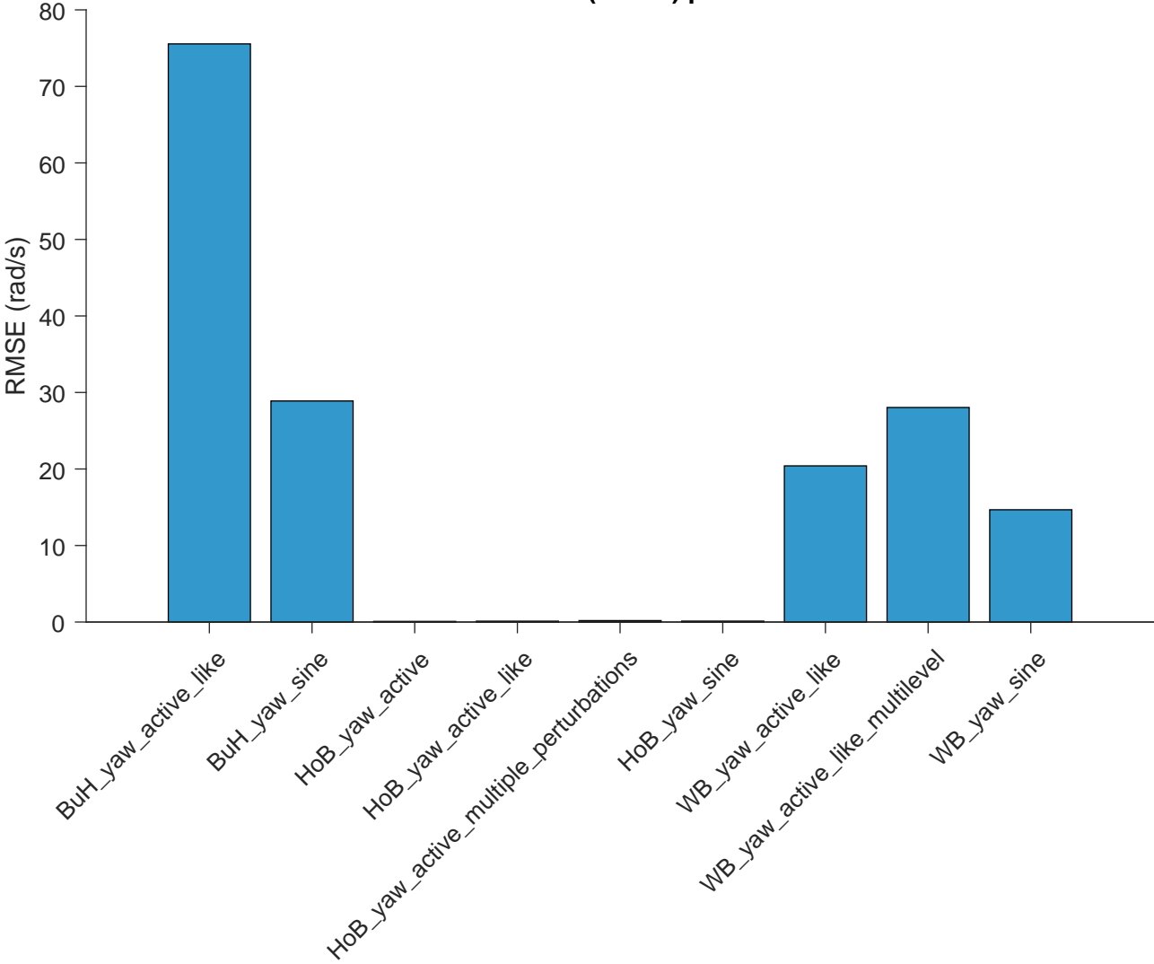
Prediction Error (RMSE) per Condition
