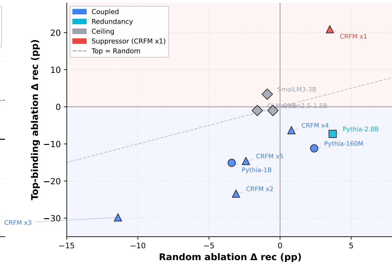
B. Top vs. Random Ablation Effect (below diagonal = top more harmful = coupled)
