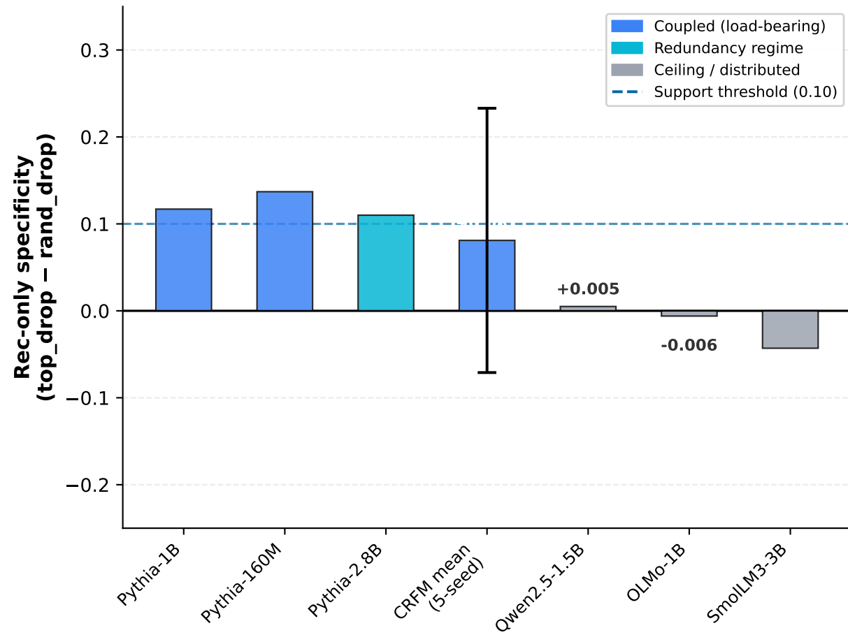
A. Causal Specificity Across Models (C5) canonical41, N=205 prompts, k=4 heads ablated
