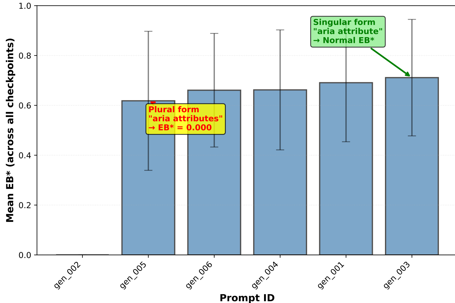
Aria Attribute: Plural Form Breaks Tokenization Systematic Zero Binding for "attributes" vs. Normal for "attribute"
