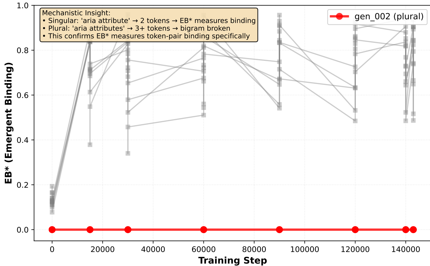
Aria Attribute EB* Trajectories Across Training Plural Form Shows Systematic Zero Binding
