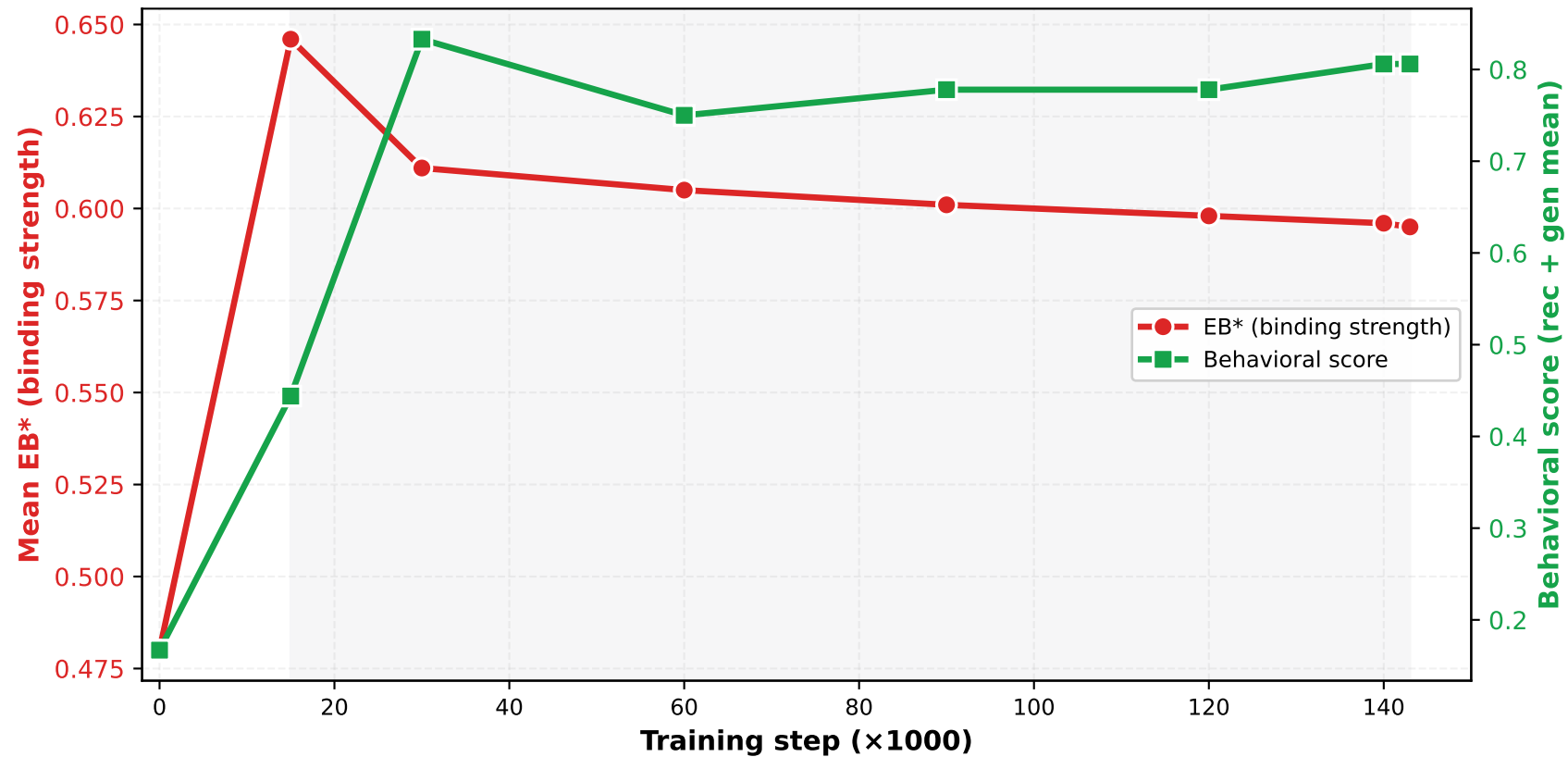
C4 Decoupling at 1B Scale: EB* Saturates While Behavior Continues Rising (Pythia-1B-deduped, 9-term mean across checkpoints)
