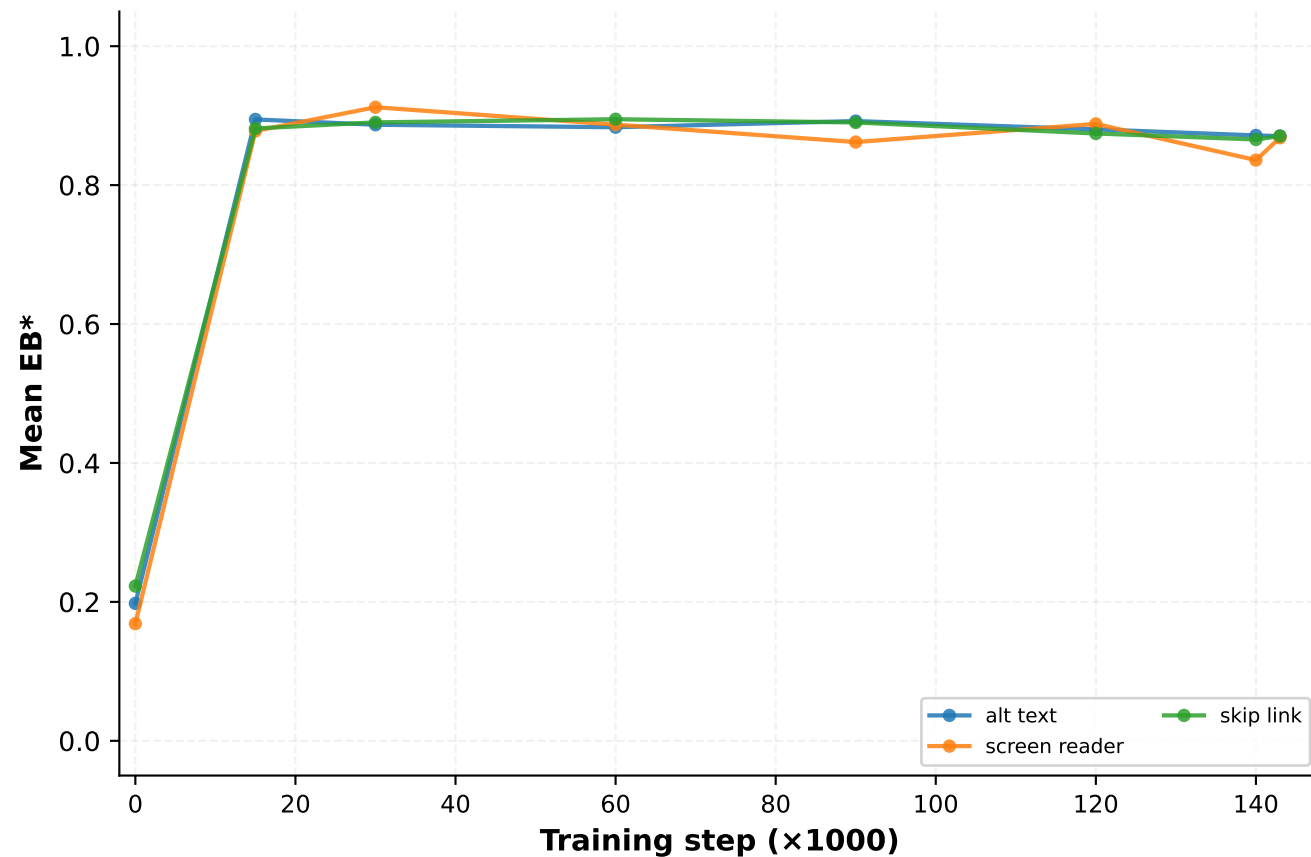
EB* Trajectories (Pythia-2.8B)
