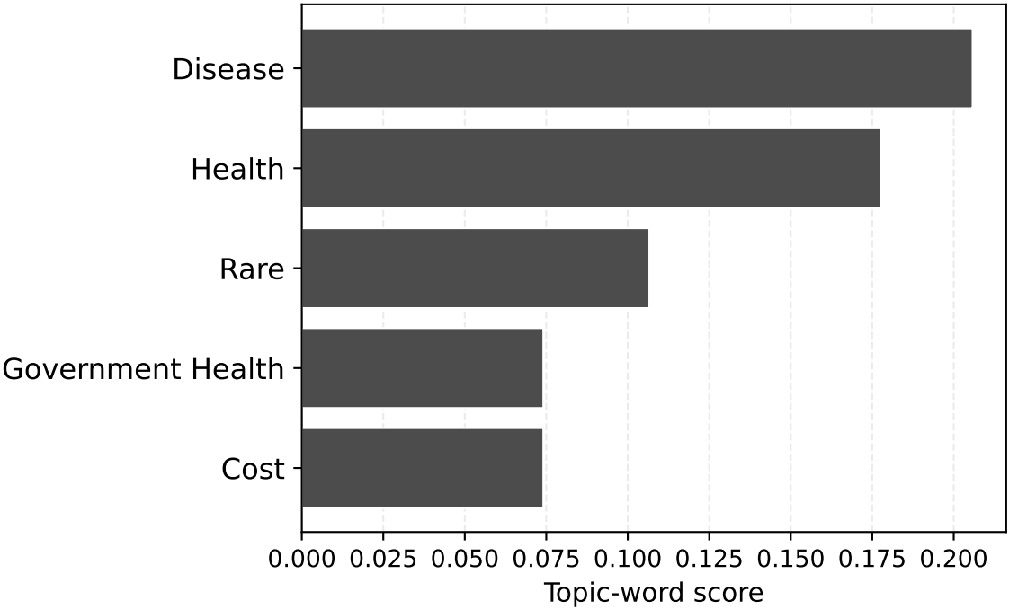
Topic 7
