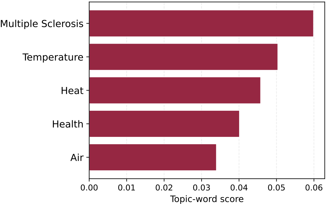
Topic 6
