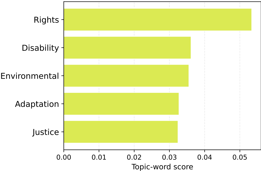
Topic 5
