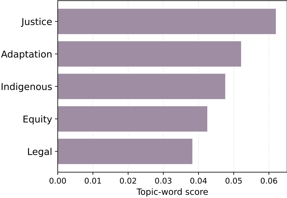
Topic 8
