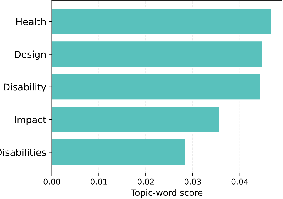
Topic 7
