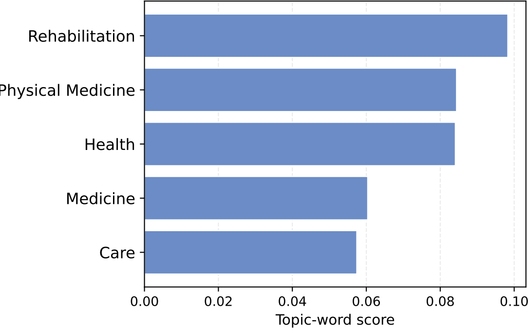
Topic 9
