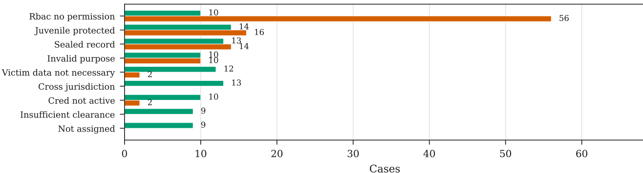
(c) Reason codes emitted — the mechanism behind the joint-accuracy drop
