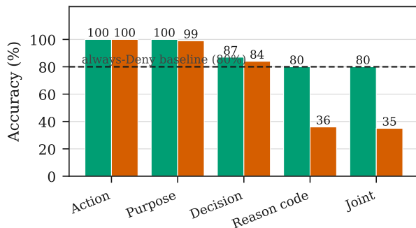
(a) Accuracy by criterion
