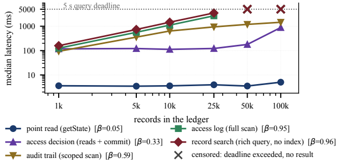
(b) Read and decision latency vs. ledger size
