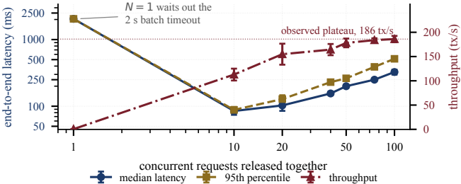
(a) Write latency and throughput vs. offered concurrency
