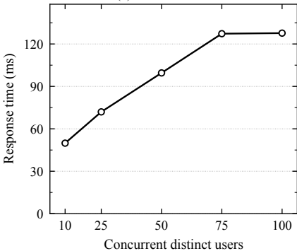
(a) Search case files
