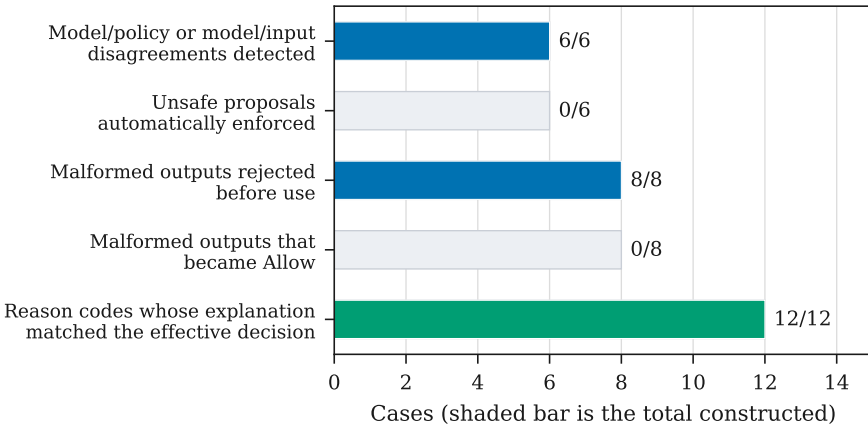
(a) Evaluated safety and explanation checks
