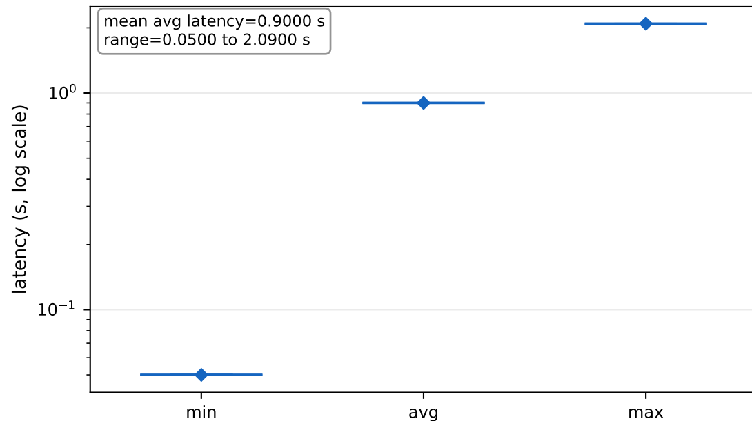
Latency metrics
