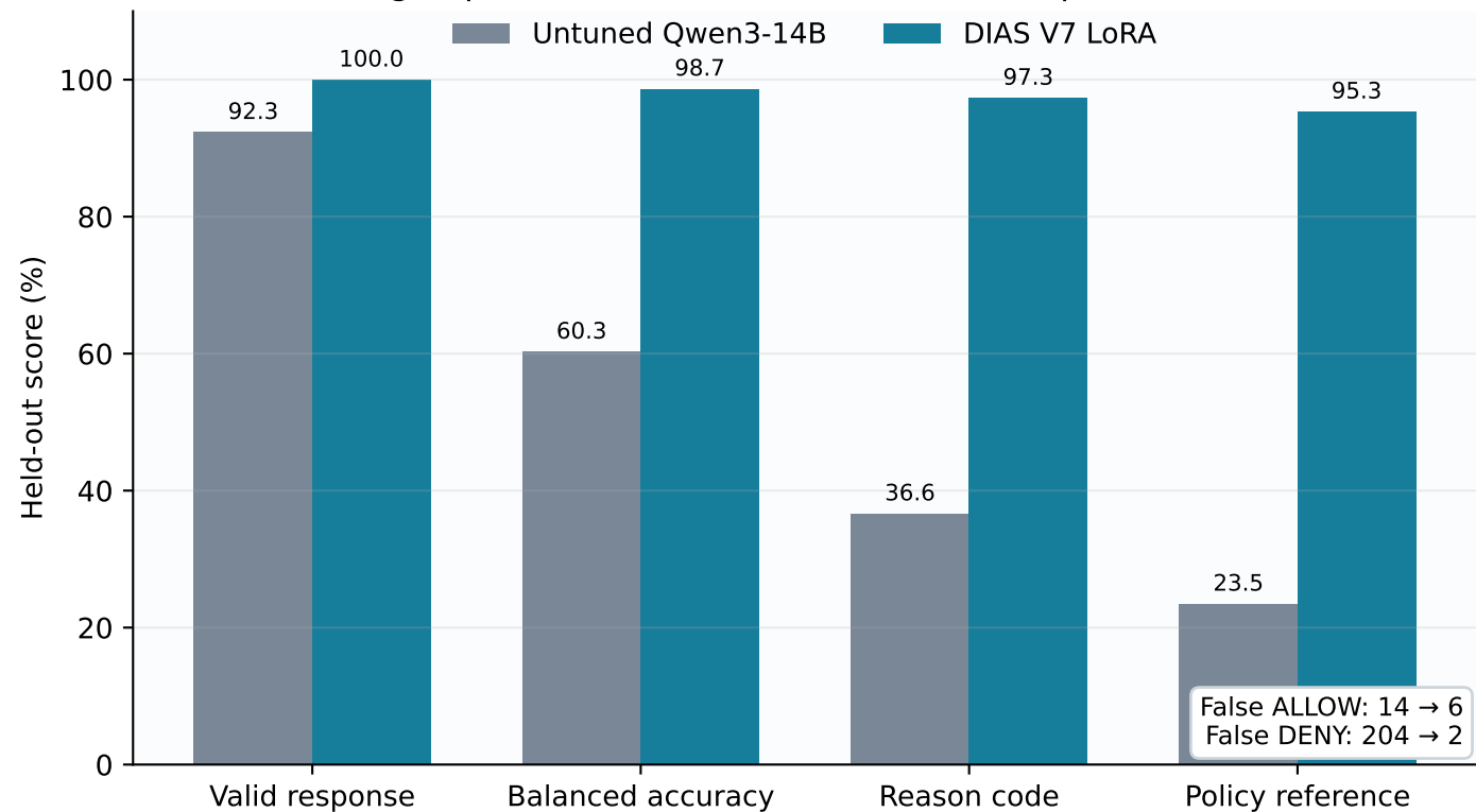
Fine-tuning improves decisions and structured explanations (n=600)
