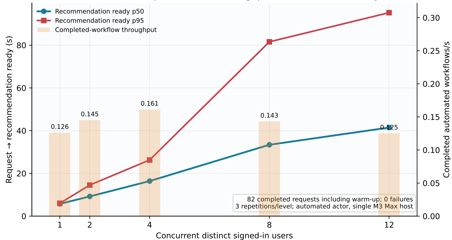
Serialized model queue bounds throughput and raises tail latency
