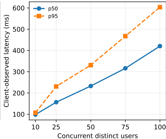
(b) Submit through commit
