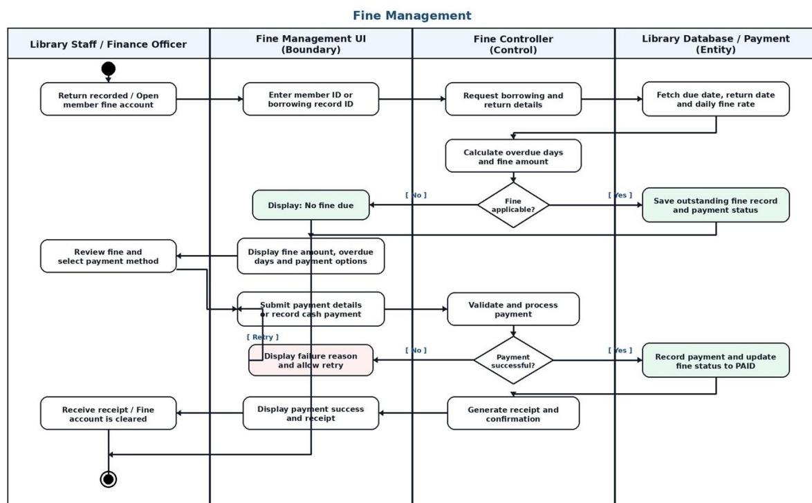
Figure 5. Activity Diagram - Manage Fines and Fine Payments
