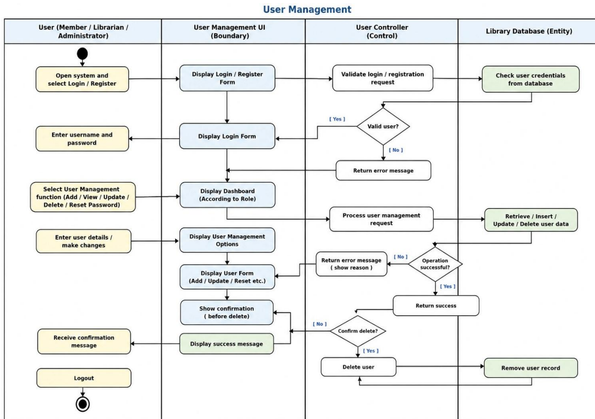
Figure 1. Activity Diagram - Manage User Accounts and Roles
