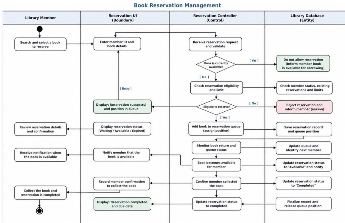
Figure 4. Activity Diagram - Manage Book Reservations
