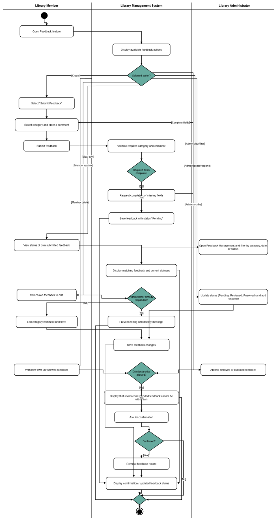
Figure 8. Activity Diagram - Manage Member Feedback
