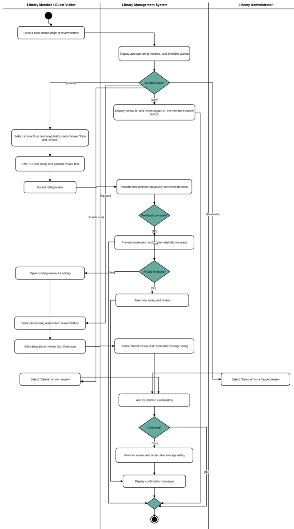
Figure 7. Activity Diagram - Book Ratings and Reviews
