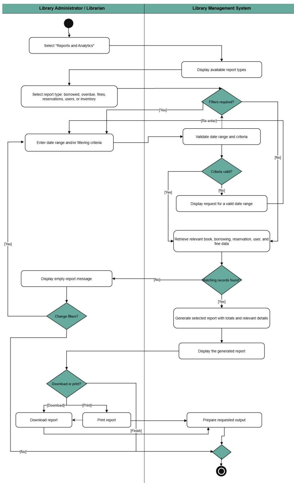
Figure 6. Activity Diagram - Generate Reports and Analytics
