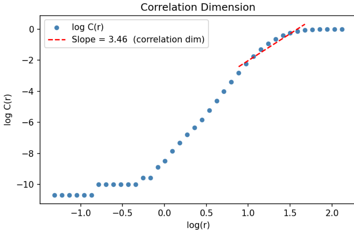
Correlation dimension - \log C(r) vs. \log(r)
