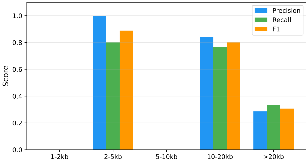
Plasmid detection by contig length
