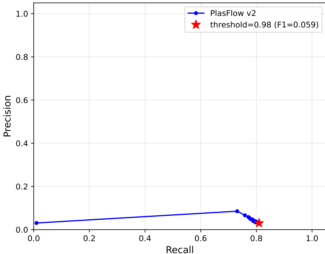
Plasmid detection: precision-recall curve
