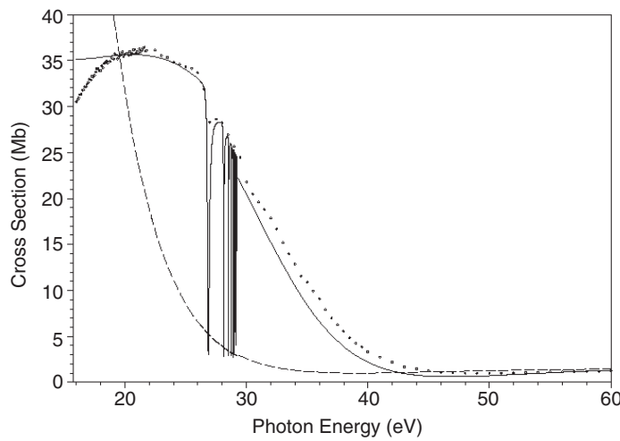
Figure 13. Total photoionization cross section of Ar. Full curve, B -spline TDLDA calculations [167]; broken curve, B -spline LDA calculations [167]; circles, experimental data [360].
