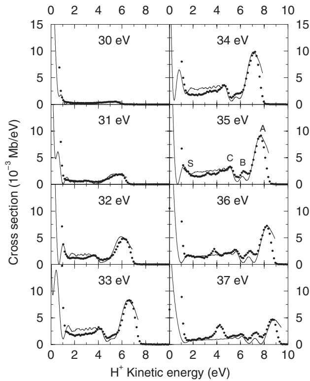
Figure 32. KED spectra of H_2 for protons detected at 90^\circ ( ^1\Pi_u contribution) [291, 292]. Full curve, theory; circles, experimental results from [456].
