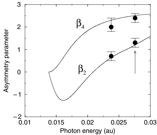
Figure 17. Asymmetry parameters \beta_2 and \beta_4 as a function of the photon energy; the theoretical results [237] are represented with the continuous curves and the filled circles with error bars represent the experimental values [428]. The arrow indicates the position of the one-photon detachment threshold.
