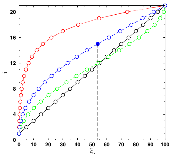
Figure A.1. Comparison of different types of breakpoint sequence: n = 21 , r_{\min} = 0 , r_{\max} = 100 . Solid curve, linear sequence. Dotted curve, exponential sequence with \gamma = 6 . Dashed curve, sinelike with \alpha = 2 . Long-dashed curve, linear-parabolic with i_0 = 15 (the connection between the parabolic and the linear sequences occurs close to r_0 = 53.8 ).
