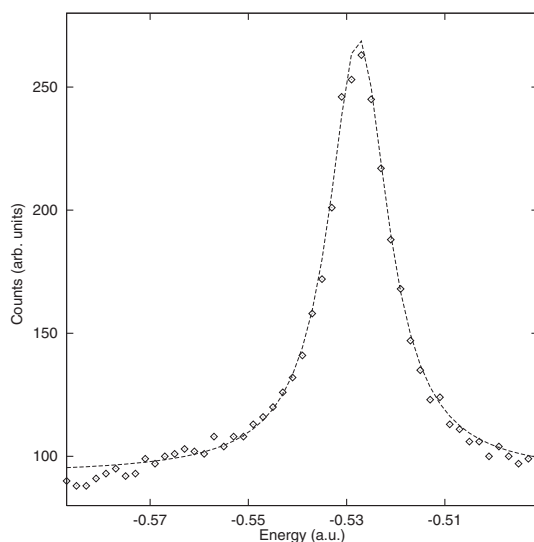
Figure 26. Histogram corresponding to the stabilization diagram shown in figure 25 [178].
