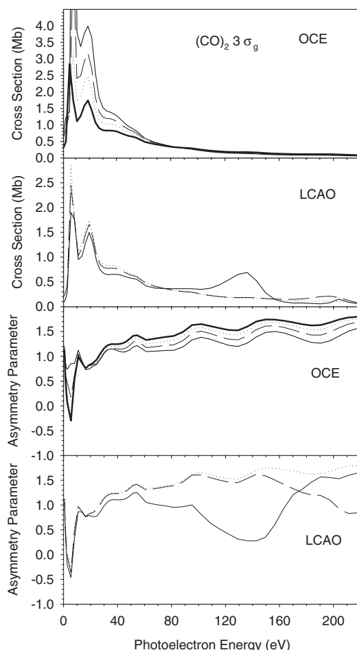
Figure 33. Convergence of OCE and LCAO photoionization parameters of (\text{CO})_2 for the 3\sigma_g orbital. OCE: (—) l_{\text{max}} = 50 , (---) l_{\text{max}} = 70 , (·····) l_{\text{max}} = 100 , convergent results are from LCAO l_{\text{max}} = 30 . LCAO: (—) l_{\text{max}} = 15 , (---) l_{\text{max}} = 20 , (·····) l_{\text{max}} = 30 .
