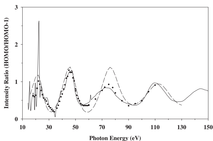
Figure 39. HOMO/HOMO -1 photoionization cross section ratio in C_{60} . Experimental data (●) and theoretical calculation (---) from [488], B -spline LDA results (—) (taken from [310]).
