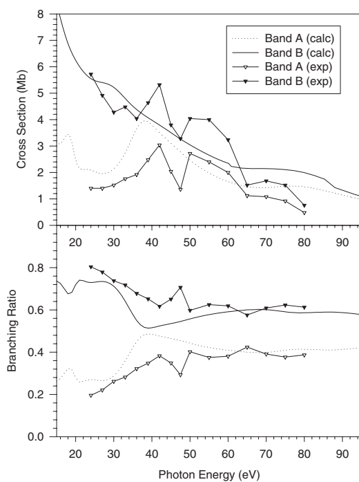
Figure 38. LDA photoionization cross sections (upper panel) and branching ratios (lower panel) relative to 8a_{1g} (band A) and 4e_{2g} (band B) orbitals in Cr(C_6H_6)_2 . Experimental data from [499] (taken from [308]).
