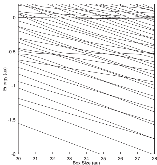
Figure 25. Stabilization diagram of H in a static field F = 0.1 \text{ MV cm}^{-1} [178].
