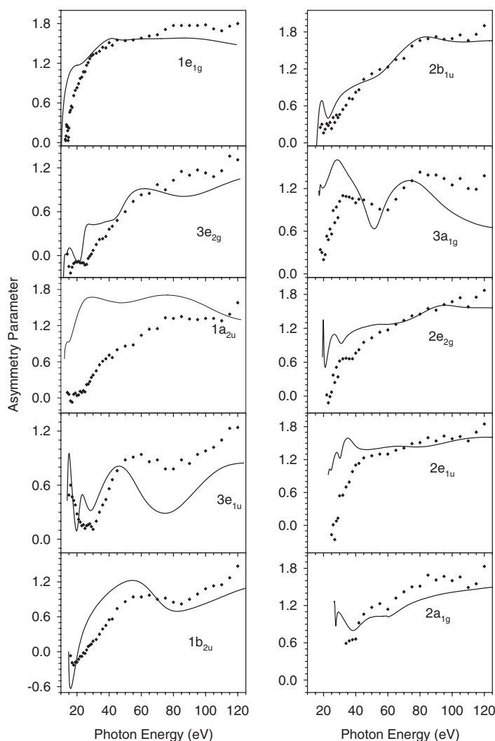
Figure 36. LDA photoionization asymmetry parameter profiles relative to all valence orbitals in C_6H_6 . (—) calculated values; full diamonds, experimental data from [496] (taken from [309]).
