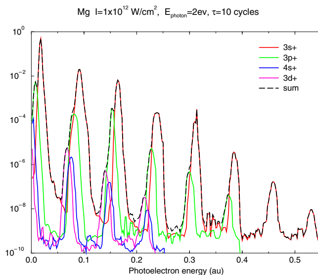
Figure 23. Photoelectron energy spectra corresponding to \text{Mg}^+ left in the ground as well as a few excited states (from [264]).
