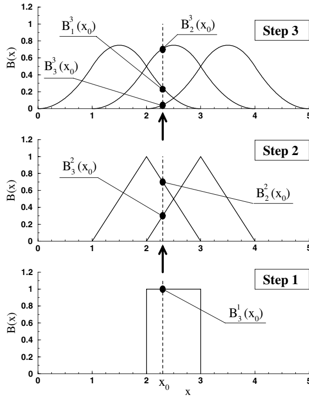
Figure 2. Recursive evaluation of B -splines up to order k = 3 , relative to the knot sequence \{0, 1, 2, 3, 4, 5\} , which are not zero at 2 < x < 3 . Each set is obtained from the previous one by applying the recursion formula (1). Notice that at each x one obtains k nonzero B -spline values, which add up to unity.
