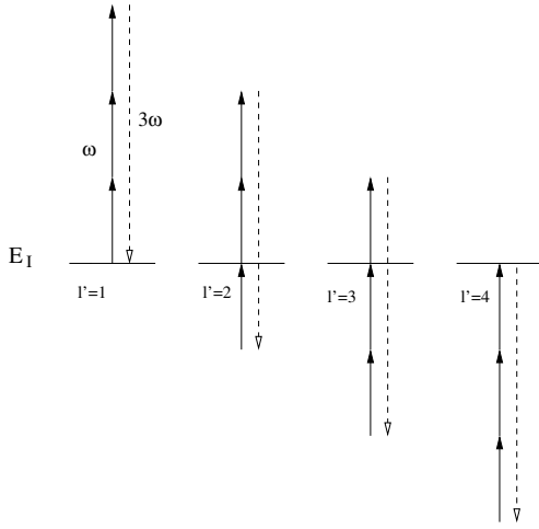
Figure 14. Schematic representation of the four different paths involved in the calculation of the nonlinear susceptibility \chi^{(3)} . The horizontal line represents the energy of the initial state E_I . Note that each l' path results in the emission of an harmonic photon of energy 3\omega , represented by a dashed arrow. The short full arrows represent the absorbed photon energy \omega .
