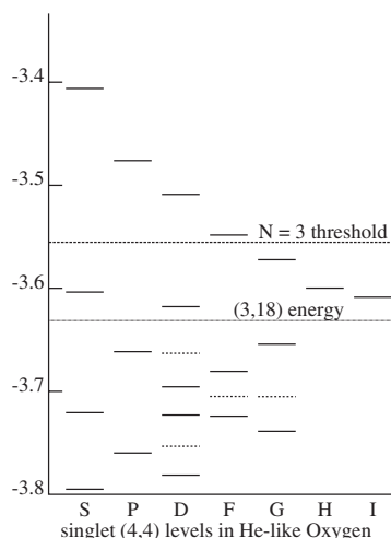
Figure 8. Positions of the singlet terms belonging to the 4l4l' complex in O^{6+} relative to the N = 3 threshold. The 3lnl' series is not included, but the average 3l18l' energy is indicated. The difference between dashed and solid lines refers to states with so-called unnatural, respectively, natural parity.
