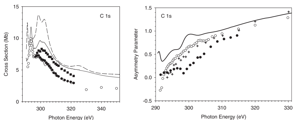
Figure 37. Left, total C 1s photoionization cross section in C_6H_6 : (---) LDA calculated profile, (—) absorption experimental data, (○) and (●) main line photoemission from two different experiments, (■) main line + satellite photoemission experimental data from [498]. Right, C 1s asymmetry parameter in C_6H_6 : (—) LDA calculated profile, (+) main line experimental data from [497], (○) main line and (●) satellite experimental data from [498] (taken from [309]).
