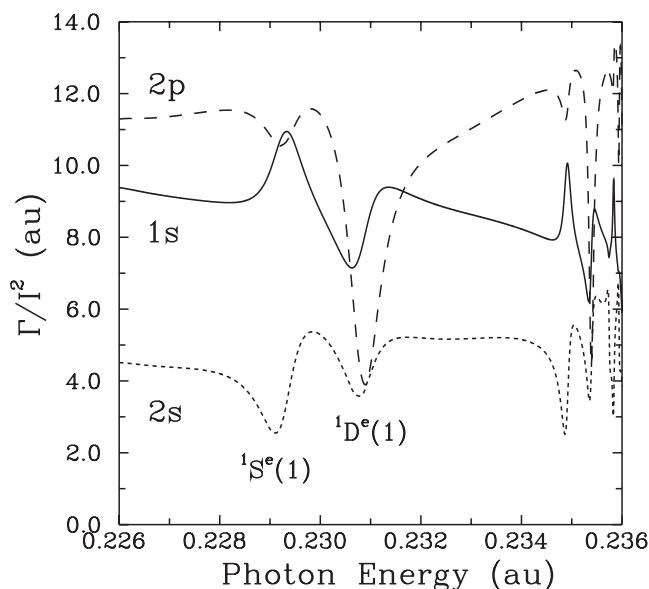
Figure 15. Partial two-photon detachment rates of \text{H}^- as a function of photon energy for \omega = 0.226\text{--}0.236 au. Labels indicate symmetry of the resonances [234].
