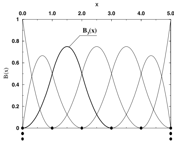
Figure 1. The full set of B -splines of order k = 3 relative to the knot sequence \{0, 0, 0, 1, 2, 3, 4, 5, 5, 5\} . Knots are represented by full circles.
