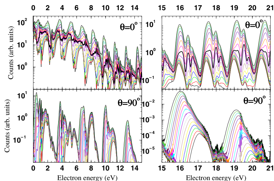
Figure 21. Theoretical low- (left) and high- (right) energy electron spectra of Ar computed at \Theta = 0^\circ and 90^\circ from the polarization axis for 16 intensities varying from 5 \times 10^{13} W cm ^{-2} up to 7 \times 10^{13} W cm ^{-2} . Black thick solid curve, I = 6 \times 10^{13} W cm ^{-2} (from [272]).
