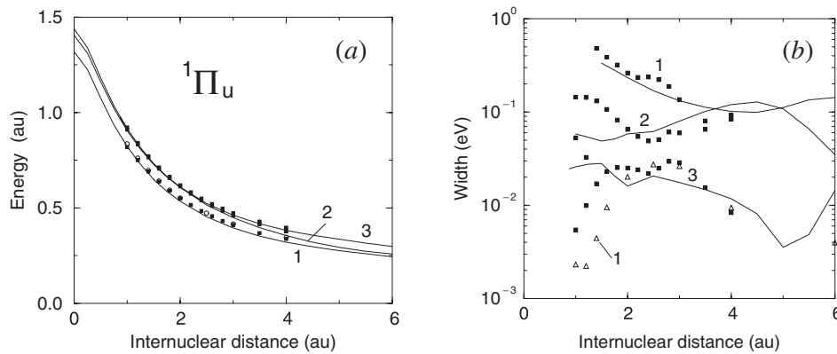
Figure 29. Theoretical energies (a) and widths (b) of the Q_2 1\Pi_u doubly excited states of H_2 . The energies are referred to the GS of H_2^+ . Solid curves, results obtained with B -spline functions [289]; open triangles, [463]; open circles, [464]; full squares, [462]. Numbers indicate energy ordering. Notice the logarithmic scale in (b).
