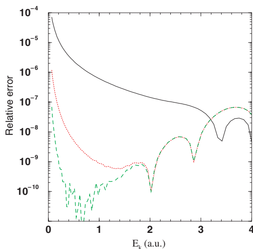
Figure 7. Relative error obtained when approximating the density of discretized continuum states with the three-point formula (equation (21)), solid curve, the five-point formula (see equations (208) of appendix A.2), dotted curve, and the seven-point formula (see equations (208)), dashed curve (linear-parabolic sequence, r_{\max} = 100 au, N = 500 B -splines and k = 7 ).
