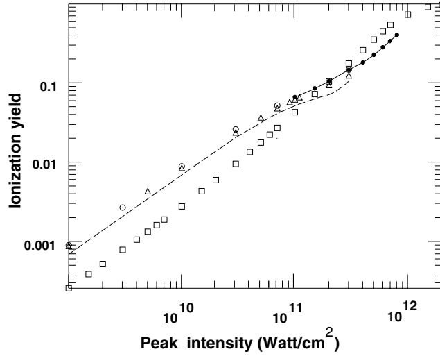
Figure 24. Ionization probability of H^- as a function of the laser peak intensity. \omega = 0.03 au, and the pulse has a cosine envelope whose FWHM is equal to four optical cycles. The open triangles are the results obtained with the B -spline functions. The open circles are those obtained with complex Sturmian functions. The open squares are from a basis calculation by Nikolopoulos et al [259]; the full circles connected by a full curve are from Scrinzi et al (see [271]). The dashed curve is obtained by integrating the R -matrix Floquet rates from Purvis et al [271] over the pulse intensity profile. (From [271].)
