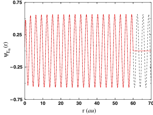
Figure 6. Comparison of a discretized continuum wavefunction (solid curve) with the exact Coulomb wavefunction (dashed curve) in H ( E_k = 54 eV, r_{\max} = 60 au).
