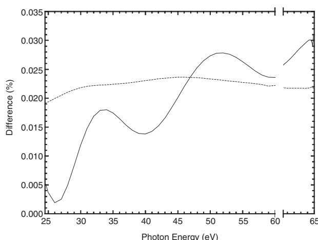
Figure 11. Percentage difference between length ( l ), velocity ( v ) and acceleration ( a ) cross sections for helium photoionization. Full curve, (l - v)/v\% ; broken curve, (v - a)/v\% .
