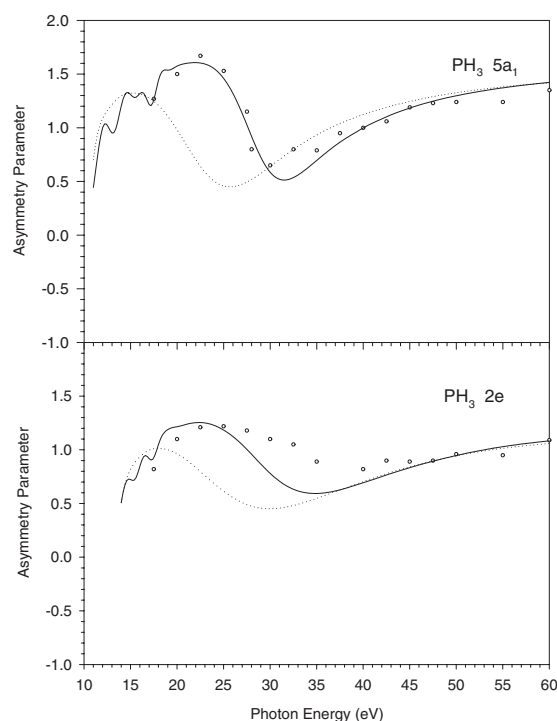
Figure 35. LDA (.....) and TDLDA (—) photoionization asymmetry parameter relative to 5a_1 and 2e orbitals in \text{PH}_3 . Experimental data (o) from [502].
