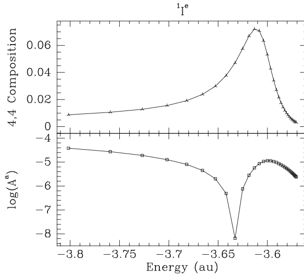
Figure 10. The effect of the interaction between a 4l4l' perturber, the 1I^e term, and a Rydberg series on the autoionization decay rates of the combined system. The amount of the perturber in the individual states is shown in the upper panel (crosses) and the corresponding autoionization rates, A in au, in the lower one (squares). Note that the maximum amount of 1I^e character in any state is less than 7%. In the Rydberg series, n \approx 13 corresponds to E \approx -3.76 au. From [210].
