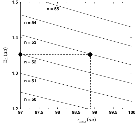
Figure 5. Plot of a selection of discretized continuum energies as a function of r_{\max} ( N = 100 ). Note that by varying r_{\max} from 97 to 98.9 au, state number 53 will scan the empty energy gap that separates it from state number 52. Note also that the curves are not straight lines but vary as 1/r_{\max}^2 .
