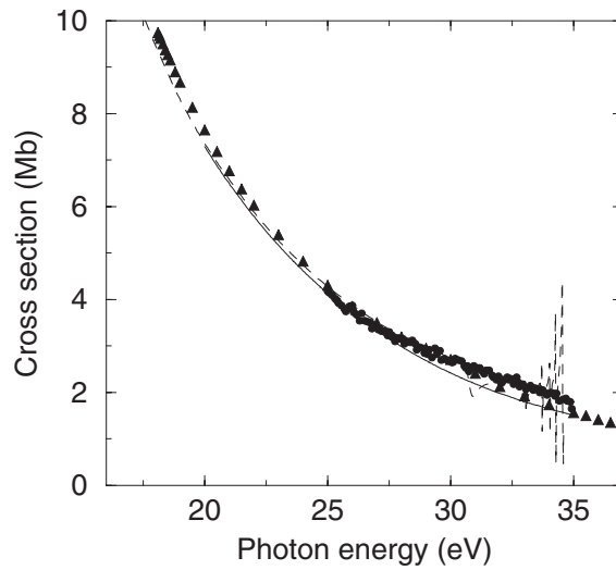
Figure 30. Total photoionization spectra of H_2 obtained with the theory of section 6.4.3 (full curve) [287] and the fixed-nucleus approximation (dashed curve) [284]. Triangles, experimental results of [468]; dots, experimental results of [469].
