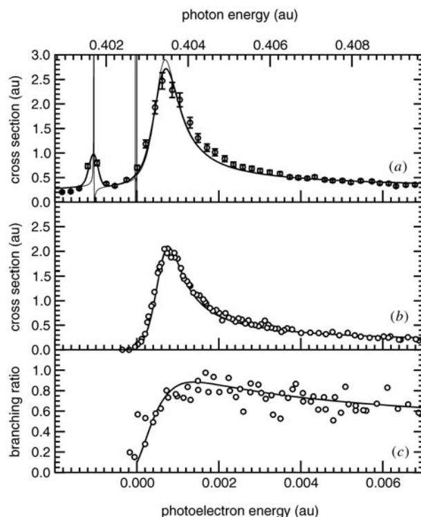
Figure 12. Comparison of B -spline calculations of Venuti and Decleva [166] with experimental data of Halka et al [355] for \text{H}^- photodetachment. The theoretical curves have been convoluted with the experimental resolution of 7 meV. Results before convolution are represented with the light line. The photoelectron energy for the n = 2 channels is indicated on the bottom axis. (a) Total cross section. (b) Partial N = 2 cross section. (c) Branching ratio \sigma_{N=2}/\sigma_{\text{total}} .
