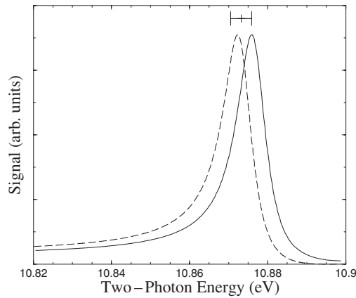
Figure 16. The yield of electrons in the two-photon detachment continuum in the region of the lowest 1D^e resonance of H^- : B -spline results from [234] (solid curve) and the best fit of experimental results (dashed curve) using the Beutler-Fano line shape [427]. We also indicate (above the shape resonance maximum) the experimental energy position of the resonance with the error bar [427].
