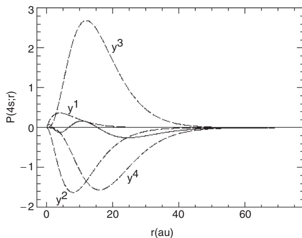
Figure 3. Expansion of the 4s wavefunction in H (solid curve) in terms of four STOs. The dashed curves represent the contribution of each orbital ( y^n = A_n r^n e^{-\alpha r} ) to the wavefunction. Note the large cancellations between the various components (from [321]).
