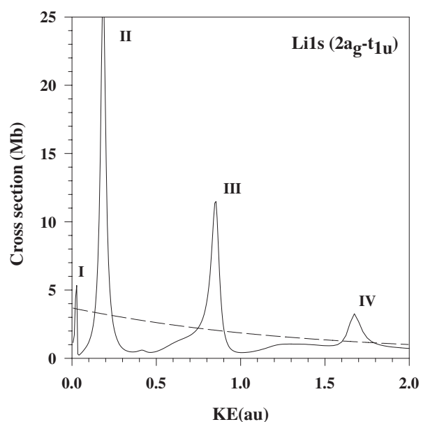
Figure 40. LDA photoionization cross section profile relative to Li 1s ionization in Li@C_{60} . (—) Li@C_{60} profiles, (---) free atom profile (taken from [303]).
