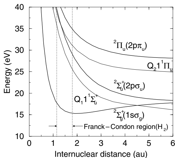
Figure 28. Potential energy curves of H_2 and H_2^+ . The curves for autoionizing doubly excited states have been taken from [285, 289]. The energy origin is placed on the lowest rovibrational level of the ground electronic state of H_2 .
