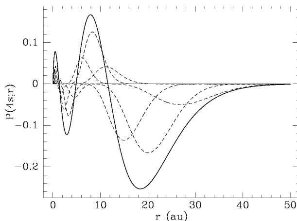
Figure 4. Expansion of the 4s wavefunction in H in terms of B -splines. The dashed curves represent the contribution of each B -spline i of order k = 5 (the terms c_i B_i(r) in equation (5)). Note here the quasi-absence of cancellations (from [321]).
