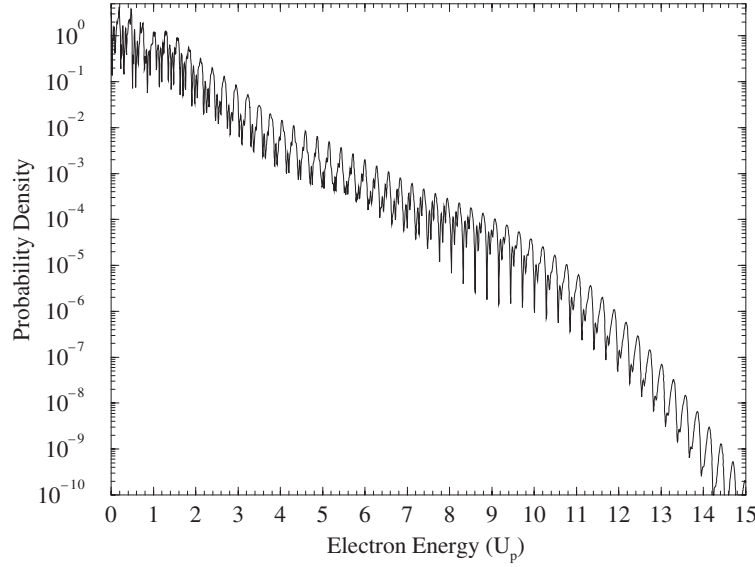
Figure 19. Angle-integrated ATI spectrum of hydrogen from [252]. \omega = 2 eV, I = 2 \times 10^{14} W cm ^{-2} , FWHM 25 fs ( U_p = 7.18 eV).
