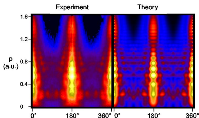
Figure 20. Comparison between theory and experiment of angle-resolved ATI spectra. The plot shows the probability as a function of the collection angle and the electron momentum. The calculation includes averaging over the interaction volume. \lambda = 800 nm, I = 7 \times 10^{13} W cm ^{-2} , FWHM 40 fs (from [446]).
