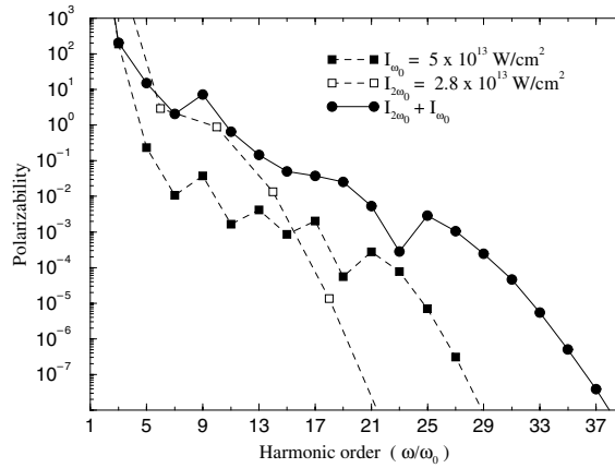
Figure 22. Comparison of the spectrum of odd harmonics produced by the bichromatic field and those obtained using each field component individually ( \hbar\omega_0 = 1.33 eV, FWHM = 50 fs, \phi = 0 ) (from [265]).
