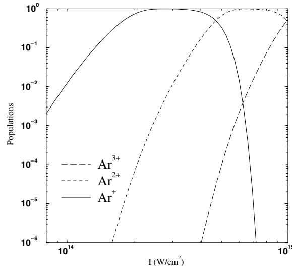
Figure 18. Probabilities for single, double and triple ionization of Ar with a 100 fs pulse as function of the laser intensity. (From [442].)
