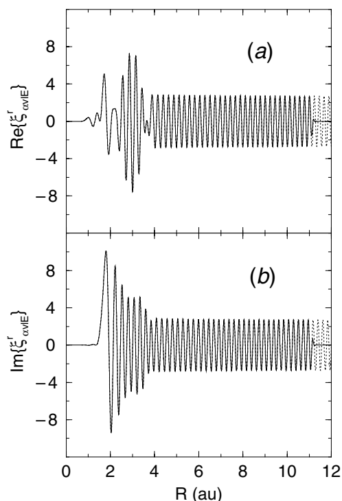
Figure 27. Nuclear wavefunction \xi_{\alpha v_{\alpha} l_{\alpha} E}^r of \text{H}_2 when the resonance r is the lowest doubly excited state of 1\Sigma_u^+ symmetry. The index \alpha represents the 2\Sigma_g^+(1s\sigma_g) state of \text{H}_2^+ , E = -0.1723 au and W_{v_{\alpha}} = -0.3824 au. The wavefunction has been obtained in the local approximation and for the dominant partial wave l_{\alpha} = 1 . Dotted curve, numerical solution of equation (170); full curve, algebraic solution in a B -spline basis of order eight with N = 240 and R_{\text{max}} = 12 au, using an absorbing potential at R = 11.5 (see text). (a) Real part; (b) imaginary part.
