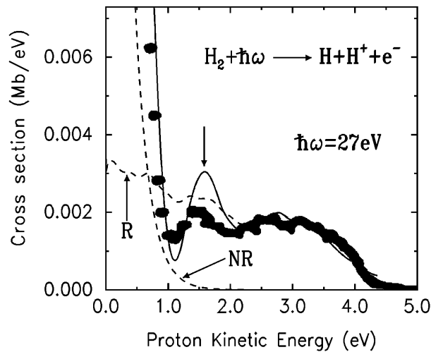
Figure 31. KED spectrum of H_2 for a photon energy of 27 eV protons detected at 0^\circ ( ^1\Sigma_u^+ contribution) [286, 288]. Full curve, theoretical results from [286]; filled circles, experimental results from [456]; dashed curves: (R) resonant and (NR) nonresonant contributions. The arrow indicates a peak not identified before [286].
