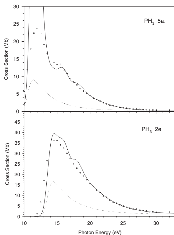
Figure 34. LDA (.....) and TDLDA (—) photoionization cross sections relative to 5a_1 and 2e orbitals in \text{PH}_3 . Experimental data (O) from [503] (taken from [306]).
