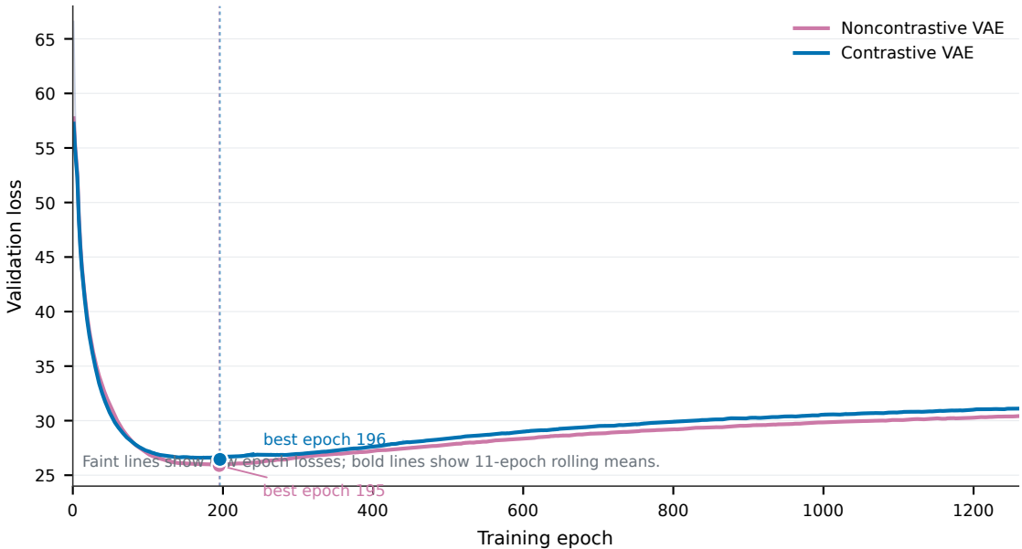
Validation-loss trajectories
