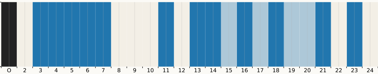
Destination tracts reached from center
