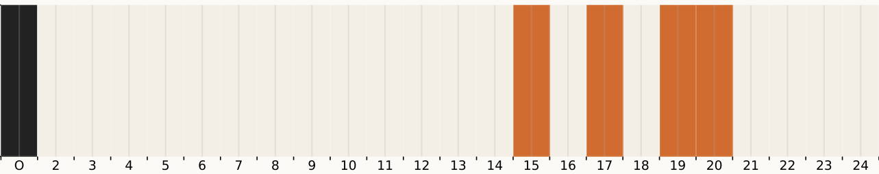
Destination tracts reached from center
