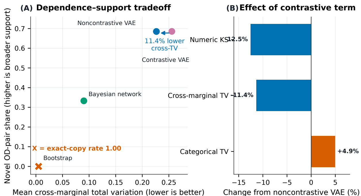
FIGURE 4 Internal trade-offs. (A) Weighted bootstrap occupies the survey-fidelity corner by exact copying; learned methods generate more rows on unseen OD pairs at the cost of larger cross-table error. (B) The contrastive term improves numeric KS and selected cross-table TV but worsens categorical TV. Only the paired cross-table improvement is significant at 0.05.
