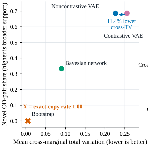
(A) Dependence–support tradeoff
