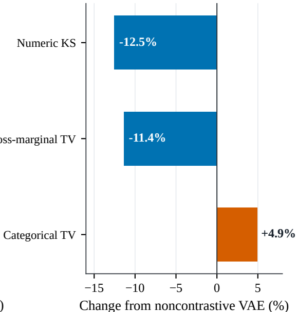
(B) Effect of contrastive term
