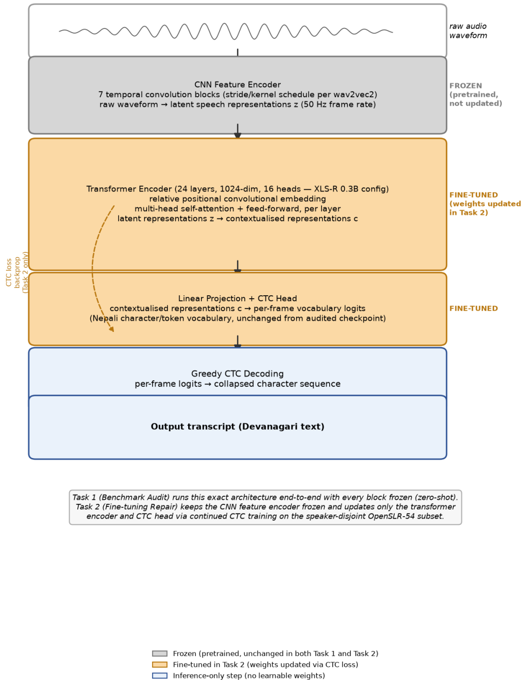
Figure 1 (reproduced). XLS-R (wav2vec2) architecture, showing the CNN feature encoder, transformer encoder, and CTC head, with frozen vs. fine-tuned components marked.
