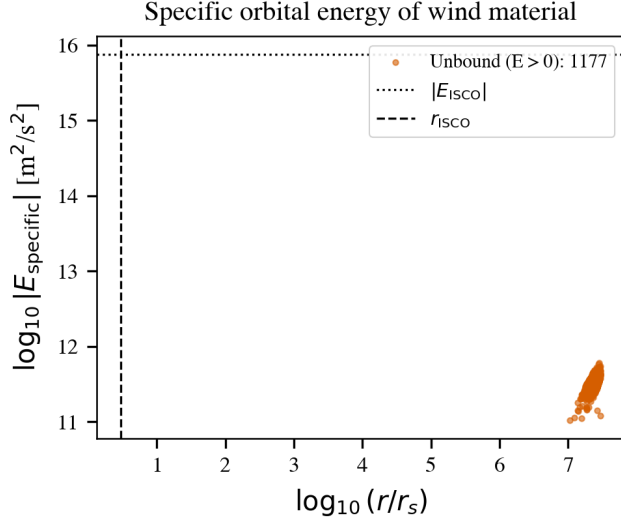
FIG. 9: Specific orbital energy diagram for all 1177 active wind superparticles, plotted as \log_{10} |E| versus \log_{10}(r/r_s) with r_s = 28.4 km for the 9.6M_\odot Gaia BH1 primary. All particles have E > 0 (unbound) and reside at r \gg r_{\text{ISCO}} = 3r_s (vertical dashed line). No particle crosses the absorbing inner boundary during the T_{\text{sim}} = 372 d integration, validating that the BHL capture rate is set by the geometry of the wind cone rather than by direct strong-field plunge [9]. Integrator: REBOUND [27], REBOUNDx gr_full [4], MERCURIUS hybrid [30], MC seed = 42.
